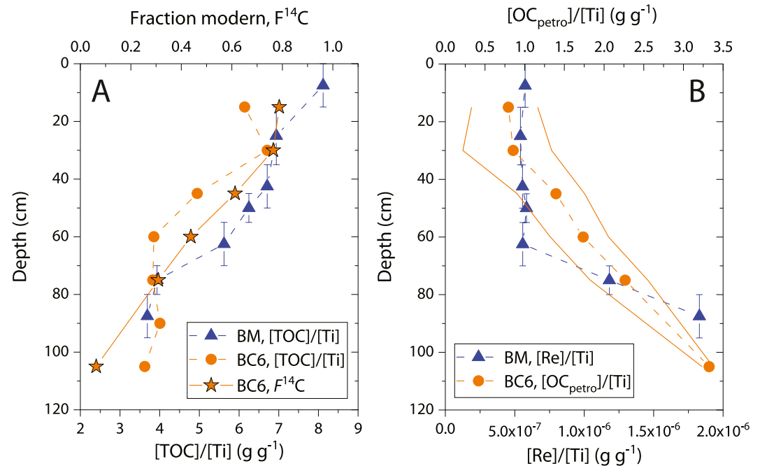
Figure 4. Weathering profiles from Bradley Creek Meadows. The two profiles BM and BC6 were collected with \sim 3 m of each other. (a) Total organic carbon concentration ( [TOC] ) normalized to titanium ( [Ti] ) from site BM (blue triangles this study) and site BC.6 (orange circles, Hsu et al., 2018), with radiocarbon measurements from BC.6 (orange stars, this study) reported as the Fraction Modern, F^{14}C . (b) Rhenium concentration ( [Re] , ppb) for site BM (black circles) and modeled rock organic carbon concentrations ( [OC_{petro}] , %) from site BC.6 (blue squares and blue lines showing \pm 1\sigma range) that derive from [TOC] and F^{14}C (Table S6 in Data Set S1).
