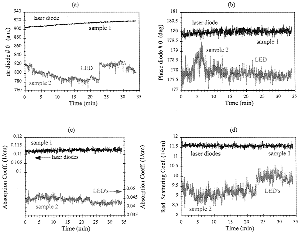
Fig. 2. Stability test performed with the old (LED's) and new (laser diodes) prototypes. The measurements were conducted on two different samples (labeled “sample 1” and “sample 2” in the figures), so that the absolute values of the readings cannot be compared. These figures compare the signal fluctuations for the (a) dc intensity, (b) phase, (c) absorption coefficient, and (d) reduced scattering coefficient. The new instrument shows a higher signal stability with respect to the old prototype.
