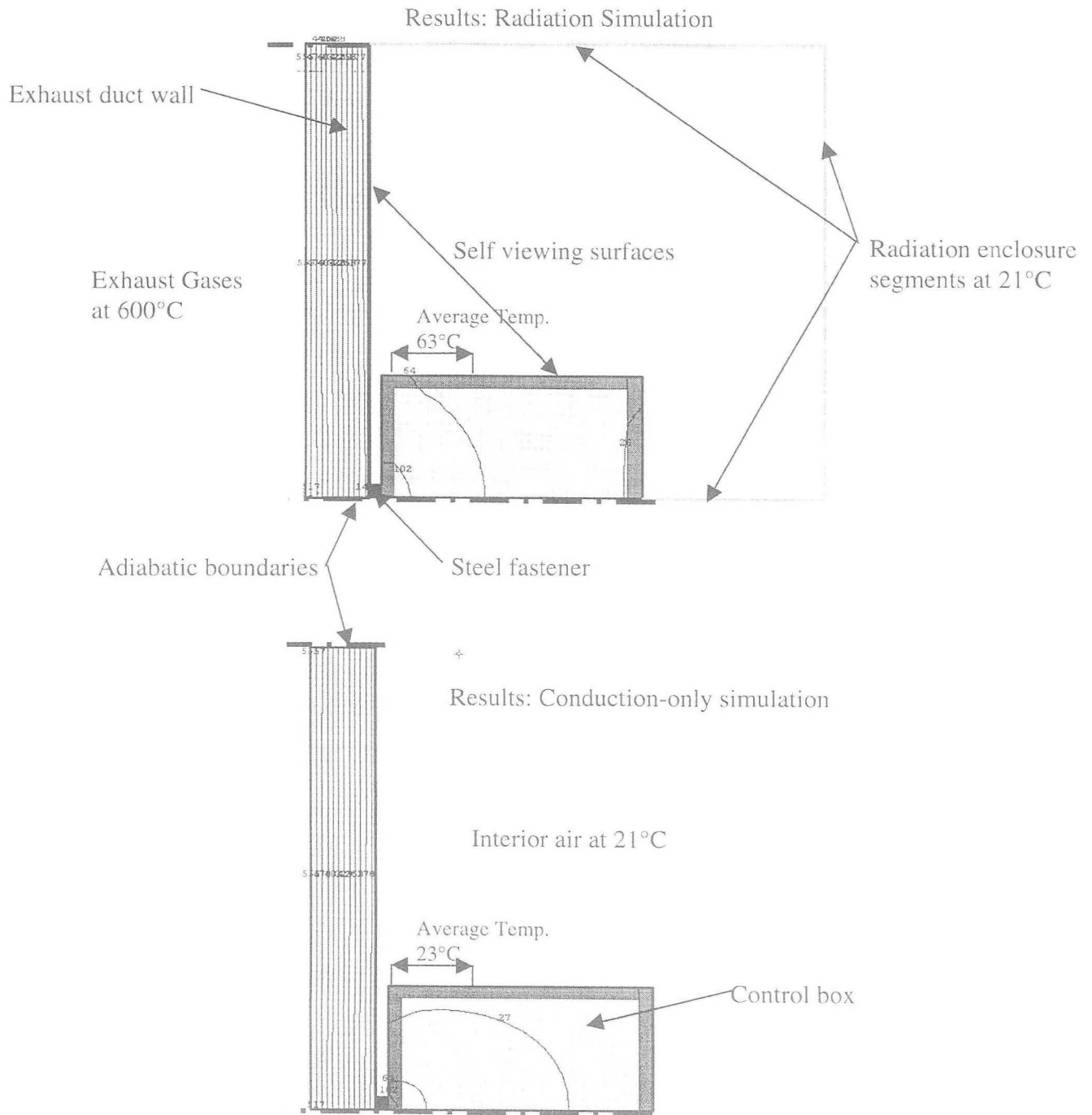
Figure 5: THERM model of a control box on a hot exhaust duct with radiation self-viewing effects modeled (top) and with self-viewing effects ignored (bottom).
