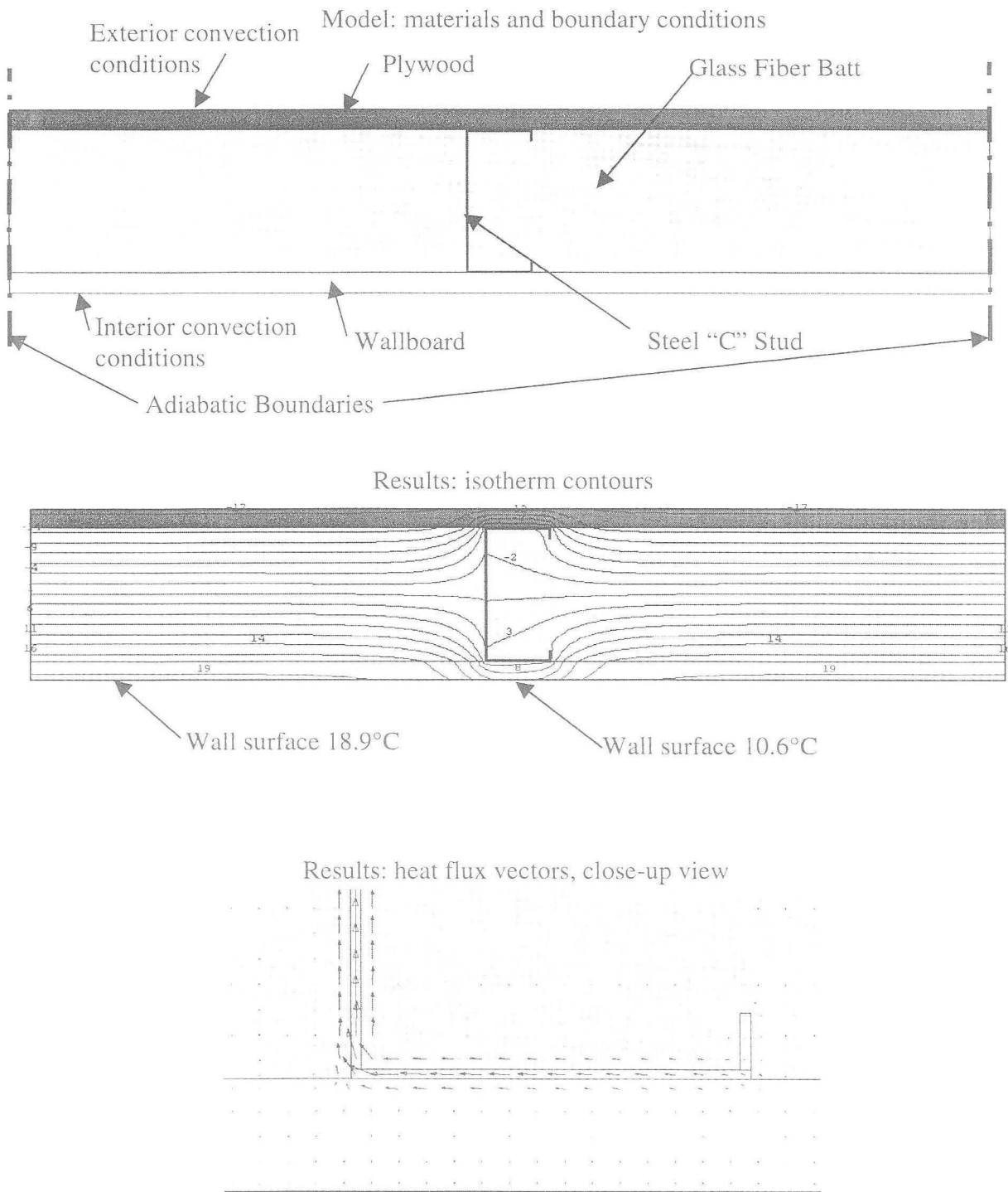
Figure 3. THERM model of an "insulated" steel stud wall: cross-section(top), results - isotherms (middle), results - heat flux vectors (bottom).
