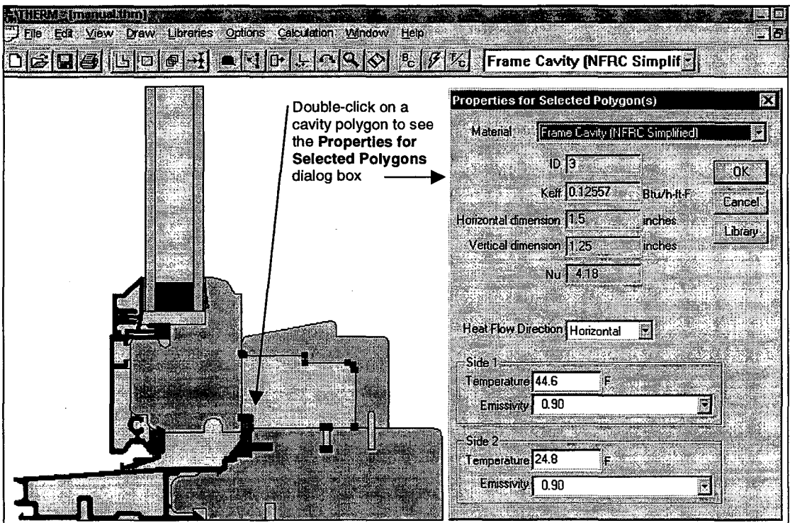
Figure 2. Assigning materials to polygons.
