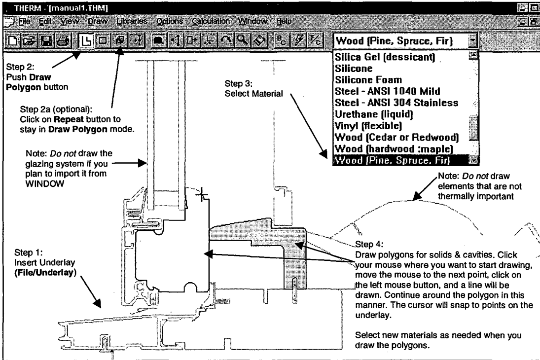
Figure 1. Drawing polygons and assigning materials.
