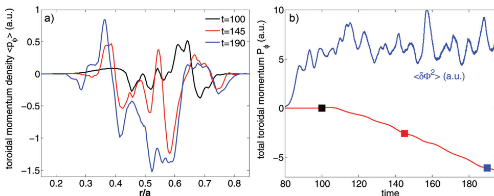
FIG. 1. (Color online) Radial profile of toroidal momentum density at three different times (left), and time history of volume-integrated toroidal momentum (with three marks corresponding to the three curves in the left panel), and turbulence intensity at a central location \rho = 0.5 (right).
