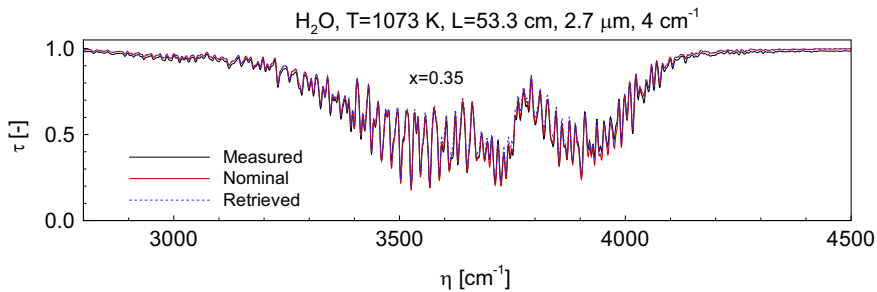
Fig. 16. Comparison of retrieved transmissivity with measured transmissivity [16] and nominal transmissivity calculated at the given temperature T=1073 K for H_2O 2.7 \mu m band.
