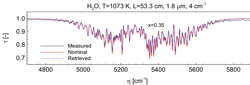
Fig. 15. Comparison of retrieved transmissivity with measured transmissivity [16] and nominal transmissivity calculated at the given temperature T=1073 K for H_2O 1.8 \mu m band.
