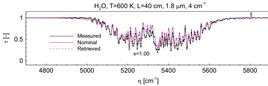
Fig. 13. Comparison of retrieved transmissivity with measured transmissivity [15] and nominal transmissivity calculated at the given temperature T=600 K for H_2O 1.8 \mu m band.
