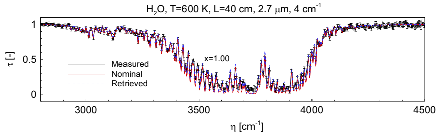
Fig. 14. Comparison of retrieved transmissivity with measured transmissivity [15] and nominal transmissivity calculated at the given temperature T=600 K for H_2O 2.7 \mu m band.
