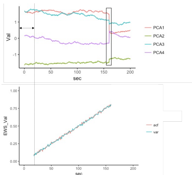
Figure 1. Audio recordings were transformed into a multidimensional feature representation, which was used to calculate putative early warning signals of critical transitions. (Top) Each single-track audio recording was transformed into a multidimensional feature representation (MFCC), then reduced to the first four principal components (colored lines). When performers transition from one soundworld to another (vertical rectangle), the performance should move to a new region of this 4-dimensional state space. (Bottom) From this 4-d representation of the audio, we calculated two putative early signals: variability and lagged autocorrelation. These were computed within a sliding window (length = 17.5 seconds), illustrated by the horizontal arrow in the top panel. In this toy example, both variability and lagged autocorrelation increase monotonically in the lead up to the critical transition.
