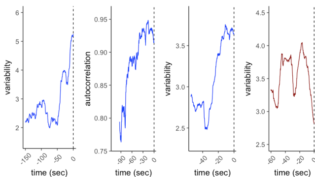
Figure 2. Early warning signals increased systematically before critical transitions. The first three plots (blue) show soundworlds where the early warning signal (vertical axis) increased systematically leading up to a musical transition (dashed lines). For comparison, the fourth plot (red) shows a soundworld where the performance did not exhibit critical
