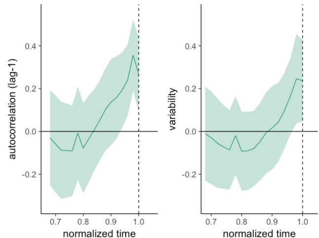
Figure 3. Mean critical slowing down in the period immediately before a musical transition (dashed line). The vertical axis indicates the direction and rate of change (i.e., Kendall's \tau ) for each early warning signal in a 35-sec. sliding window ending at that moment. Positive values indicate monotonic increase. Time (x-axis) is normalized to go from 0 to 1 within each soundworld. Error ribbon = standard error of the mean.
