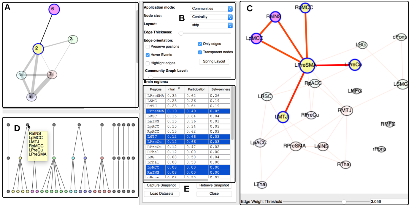
Fig. 6. A) The community graph highlights the subcommunities associated with the community selected in the dendrogram view. B) Configuration options provide various choices for interactivity, such as toggling hovering/clicking, choosing graph layout and varying the opacity of highlighted nodes. C) The brain region graph displays highlighted nodes associated with selected sub communities. D) (While the dataset is same as Fig. 1F, the threshold value for this visualization view is different) The dendrogram view displays the hierarchy of communities. The communities that do that not have any edges emanating from them are grayed out. E) A table view lists important graph properties of the graph shown in Fig. 7C.
