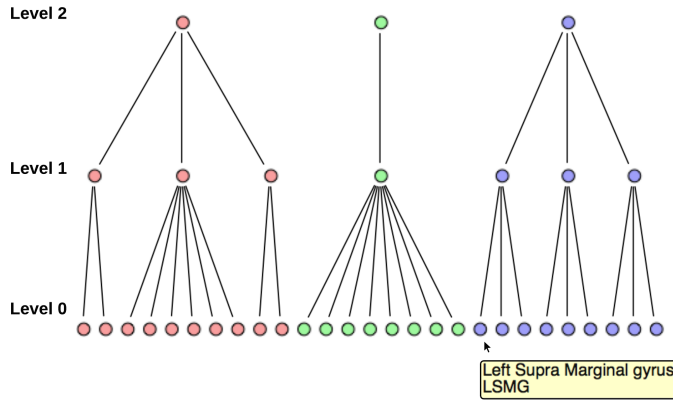
Fig. 5. The dendrogram view shows the hierarchical modular information of a community corresponding to threshold value 3.309. Level 1 of the dendrogram represents sub-communities formed when optimizing modularity locally with the nodes in level 0; level 2 nodes represent the final community emerging from the sub-communities identified in level 1.
