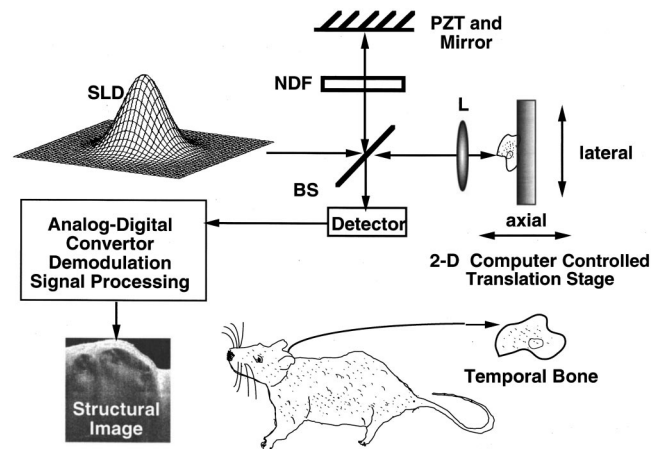
Fig. 1 Schematic of OCT imaging system: SLD—superluminescent diode, BS—beam splitter, PZT—piezoelectric transducer and mirror, NDF—neutral density filter, and L—lens.
