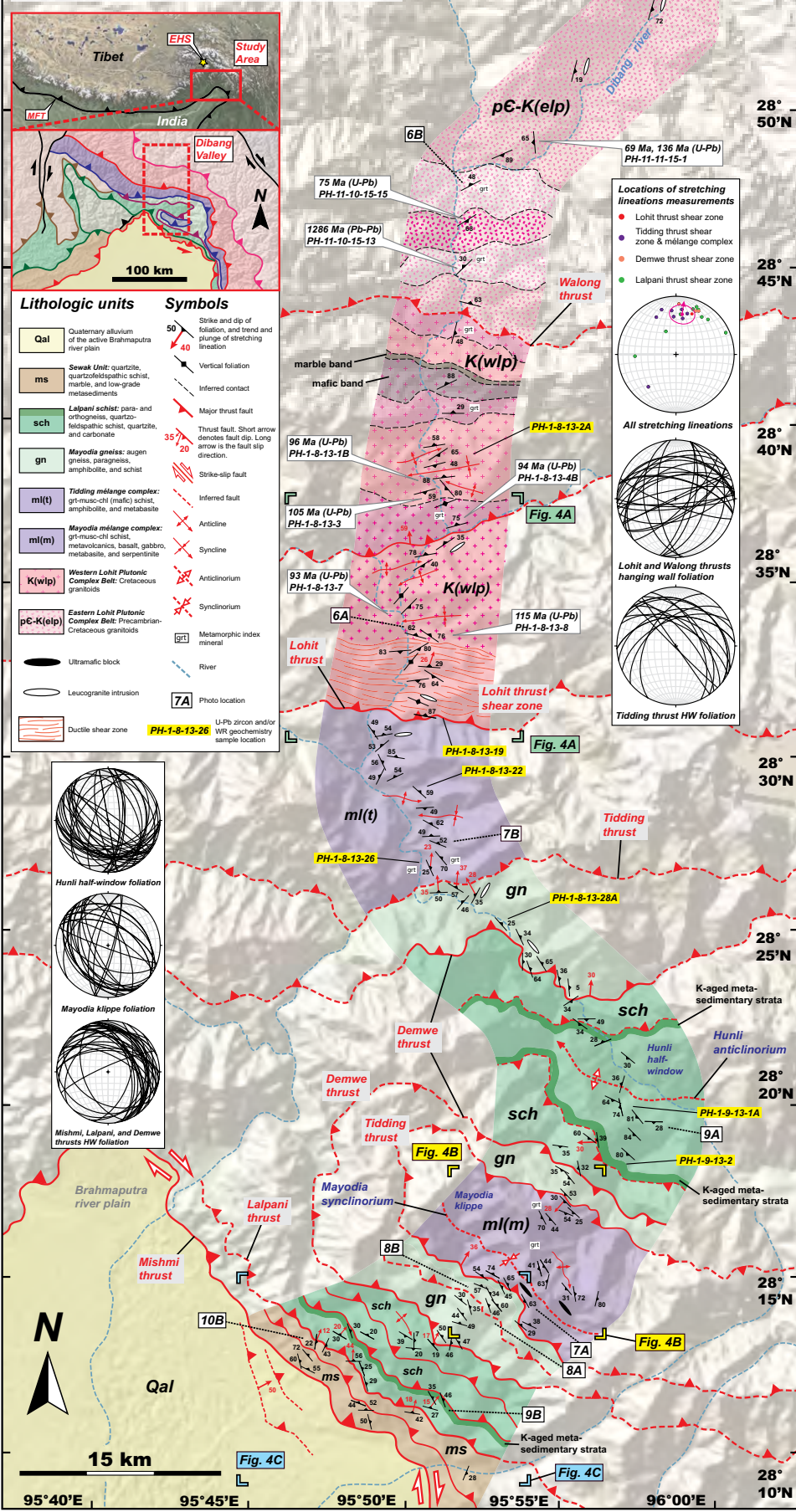
Figure 3. Geologic map of Dibang Valley modified from Haproff et al. (2018). See Figure 4 for additional sample locations. Abbreviations: EHS—eastern Himalayan syntaxis; HW—hanging wall; MFT—Main Frontal thrust; and WR—whole-rock.
