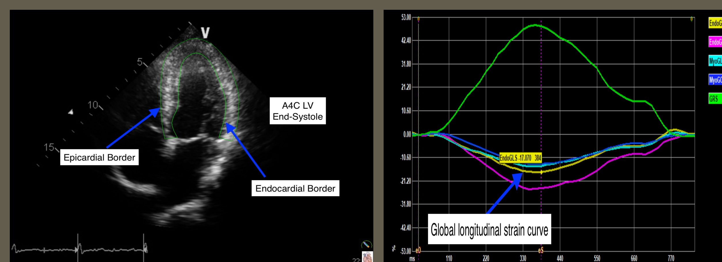
Figure 1. A4C Characterization of LV GLS function. To derive LV strain curves, the ROI was selected at the base of the mitral valve leaflet for both end-systole and end-diastole measurements (A, B). After aligning the tracing to match with the endocardial border, epicardial borders were adjusted to encompass the thickness of the myocardium. The generated strain curve (C) displays the GLS (%) versus time (ms) in yellow. Each colored line represents corresponding strain measurements such as GCS, and GRS. Similar techniques were used to generate strain curves for RA, RV, and LA chambers.
