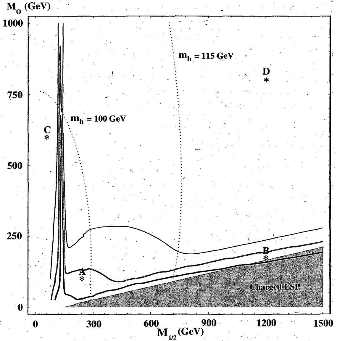
Figure 1: Preferred Dark Matter Region for cMSSM. Contours of \Omega_{\chi} h^2 of 0.1 (bottom-most contour), 0.3 and 1.0 (top-most contour) are given. The shaded region is ruled out by virtue of having the stau as the LSP. The Higgs pole region and stau coannihilation tail are clearly discernible. We have also added contours of constant Higgs mass for m_h = 100 GeV, and m_h = 115 GeV. The four labeled points are examined in Figure 2.
