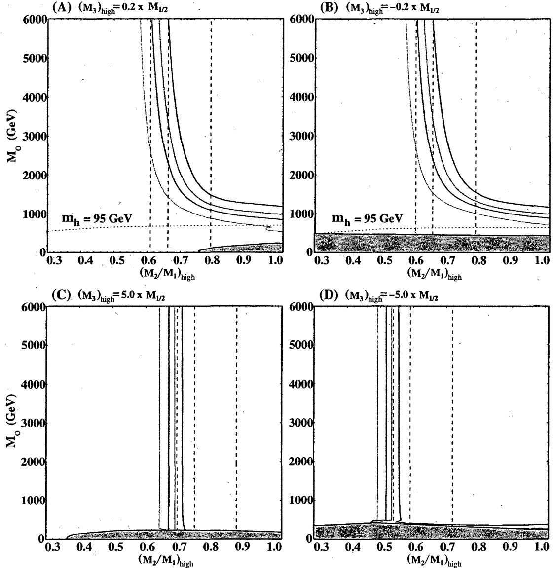
Figure 7: Preferred Dark Matter Region with Nonuniversal Gaugino Masses for Differing Signs of M_3 . The solid lines are lines of constant \Omega_\chi^2 and the dashed lines represent values of (M_2/M_1)_{\text{low}} = 1.15, 1.25 and 1.50 as in Figure 6. The shaded regions are excluded by virtue of having a stau for the LSP. We have indicated the Higgs mass constraint in panels (A) and (B). Here M_{1/2} is taken to be 500 GeV in all panels.
