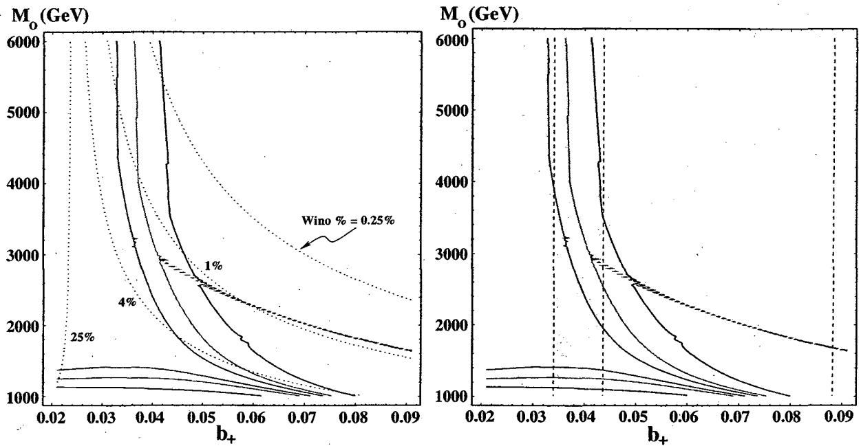
Figure 10: Preferred Region in the BGW Model. Contours of constant relic density are given as in Figure 8 by the solid lines for \Omega_\chi h^2 = 0.1, 0.3, \text{ and } 1.0 only. The left plot gives dotted lines of constant wino content (25%, 4%, 1%, 0.25% from left to right). The right plot gives dashed lines of constant ratio (M_2/M_1)_{low} (1.15, 1.25, 1.5 from left to right).
