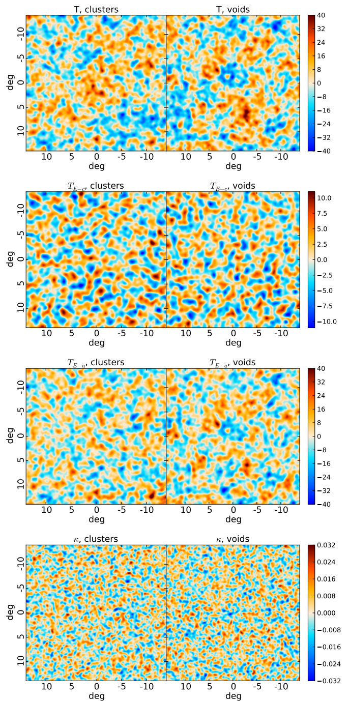
Fig. 10. Stacked patches of the scalar components from the SEVEM solution, at the supercluster (first column) and supervoid (second column) positions from GR08. From top to bottom: T , T_{E-c} , T_{E-u} and \kappa components. Temperature maps are given in \mu\text{K} units.
