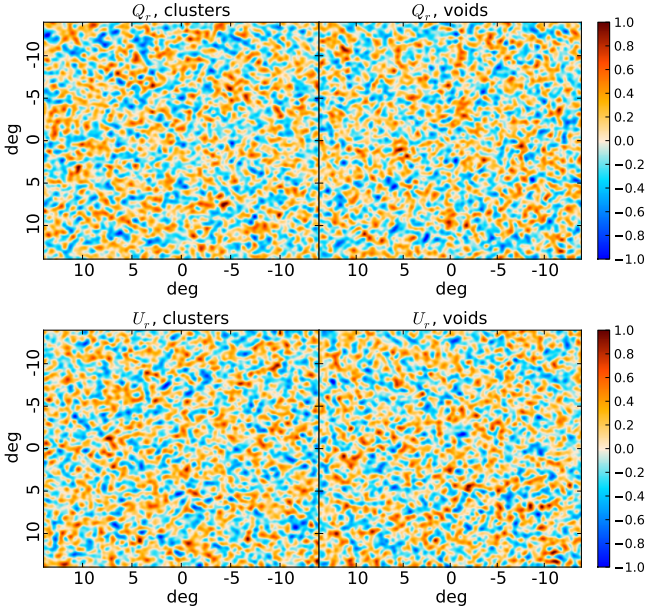
Fig. 11. Stacked patches of the Q_r (top) and U_r (bottom) components from the SEVEM solution in \mu\text{K} , at the supercluster (first column) and supervoid (second column) positions from GR08.
