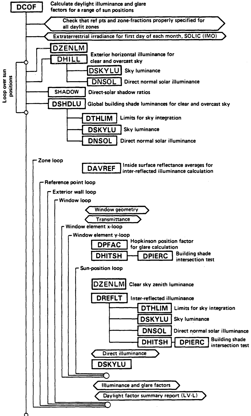
Fig. 6. Flowchart for DOE-2.1B daylighting preprocessor. Daylighting subroutines are in boldface.
