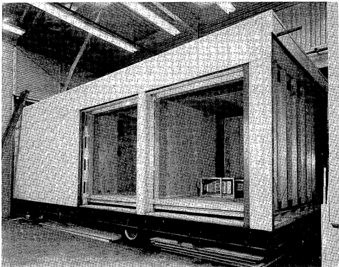
Fig. 11. Exterior view of Mobile Window Thermal Test (MowITT) facility showing the side-by-side test chambers.
