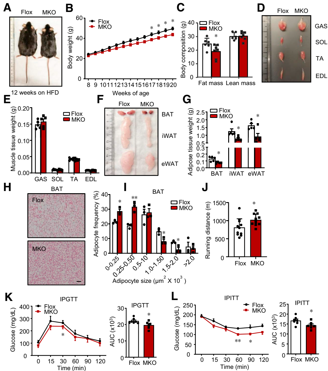
Figure 3 —Mice with IRF4 ablation in skeletal muscle are resistant to HFD-induced obesity. A : The morphology of male MKO and Flox mice on 12-week HFD. B : The body weight of male MKO and Flox mice on HFD ( n = 8 – 10 ) ( *P < 0.05 ). C : The body composition of male mice from A ( n = 6 – 7 ) ( *P < 0.05 ). D : The morphology of GAS, soleus (SOL), tibialis anterior (TA), and extensor digitorum longus (EDL) in male MKO and Flox mice on 12-week HFD. E : The weight of GAS, soleus, tibialis anterior, and extensor digitorum longus in male MKO and Flox mice on 12-week HFD ( n = 5 ). F : The morphology of BAT, iWAT, and eWAT in male MKO and Flox mice on 12-week HFD. G : The weight of BAT, iWAT, and eWAT from mice on 12-week HFD ( n = 5 ) ( *P < 0.05 ). H : Hematoxylin-eosin staining and adipocyte number of BAT in male MKO and Flox mice on 12-week HFD (scale bars, 50 \mu\text{m} ). I : The adipocyte frequency of different adipocyte size of BAT from H ( n = 3 ) ( *P < 0.05 and **P < 0.01 ). J : The running distance of male MKO and Flox mice ( n = 10 – 11 ) ( *P < 0.05 ). K and L : GTT and ITT in male MKO and Flox mice ( n = 6 – 7 ) ( *P < 0.05 and **P < 0.01 ). All results are expressed as means \pm SEM. IPGTT, intraperitoneal GTT; IPITT, intraperitoneal ITT.
