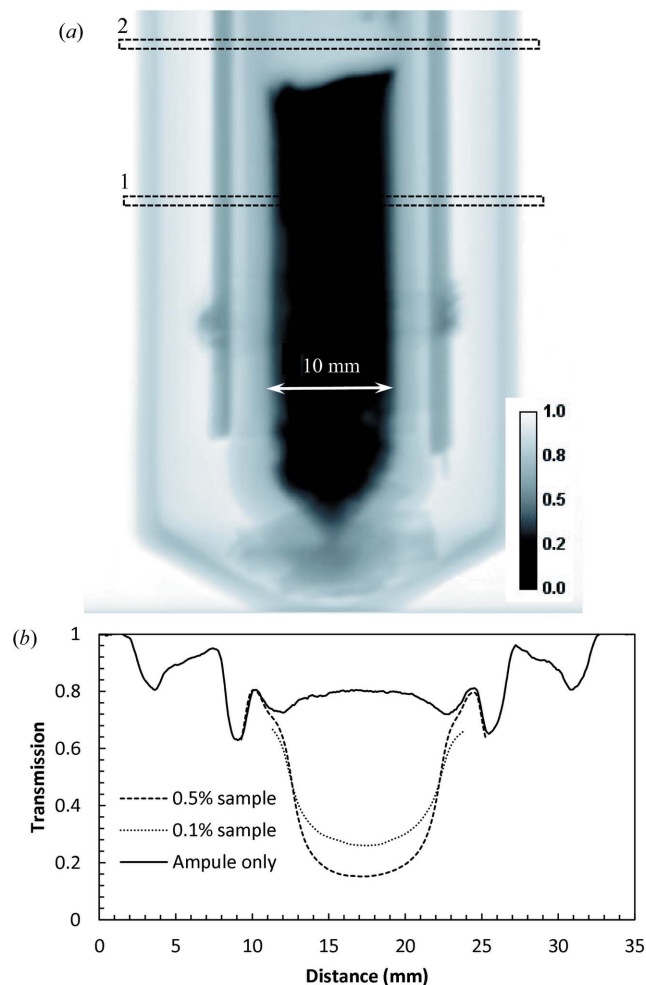
Figure 6 (a) A neutron transmission image of the BaBrCl:0.5%Eu sample with the heat absorbers mounted on the exterior of the sealed silica glass tube. BOA beamline, \sim 2 min integration, original charge sample, measured at room temperature. (b) Cross sections through the image areas shown by the dashed rectangles.
