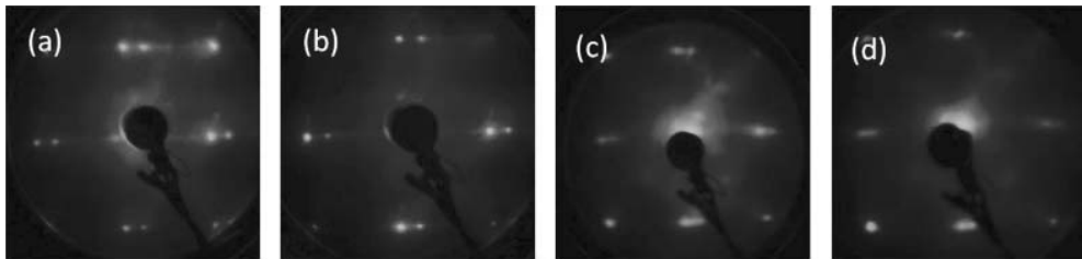
FIG. 1. (Color online) LEED patterns taken at \sim 123 eV at each stage of the FeMn(10ML)/Fe(2ML)/Co(20ML)/Cu(1,1,10) sample growth. (a) Cu(1,1,10) substrate, (b) after 20 ML Co growth, (c) after 2 ML Fe growth, and (d) after 10 ML FeMn growth.
