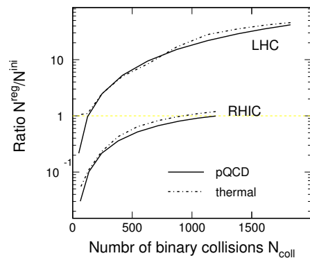
FIG. 4: The ratio of regenerated to initially produced J/\psi yields at RHIC and LHC energies in pQCD and thermal scenarios. At the LHC, we choose \sigma_{pp}^{\Psi} = 18.9 \mu\text{b} [32], \sigma_{pp}^{c\bar{c}} = 5740 \mu\text{b} [33], \tau_0 = 0.3 \text{ fm} and initial temperature 680 \text{ MeV} .
