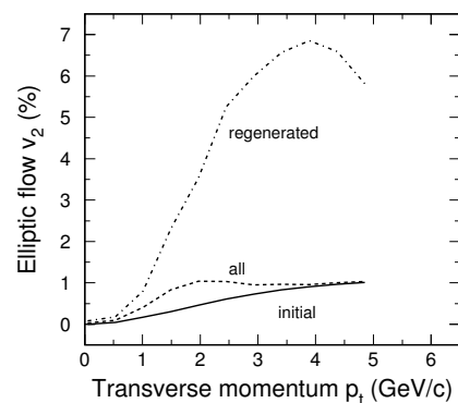
FIG. 3: The J/\psi elliptic flow in \sqrt{s_{\text{NN}}} = 200 \text{ GeV Au} + \text{Au} collisions at impact parameter b = 7.8 \text{ fm} . The calculations are the same as in Fig. 1.
