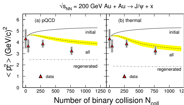
FIG. 2: The J/\psi averaged transverse momentum square as a function of the number of binary collision, N_{\text{coll}} . The calculations are the same as in Fig. 1. The PHENIX [30] data are shown.
