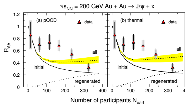
FIG. 1: The nuclear modification factor R_{AA} as a function of participant number N_{part} in pQCD (a) and thermal (b) charm quark distributions. The solid and dot-dashed curves are the calculations with only initial production and only regeneration. The bands are the full result, including the uncertainty in initial charm quark and \Psi production. The data are from PHENIX [30].
