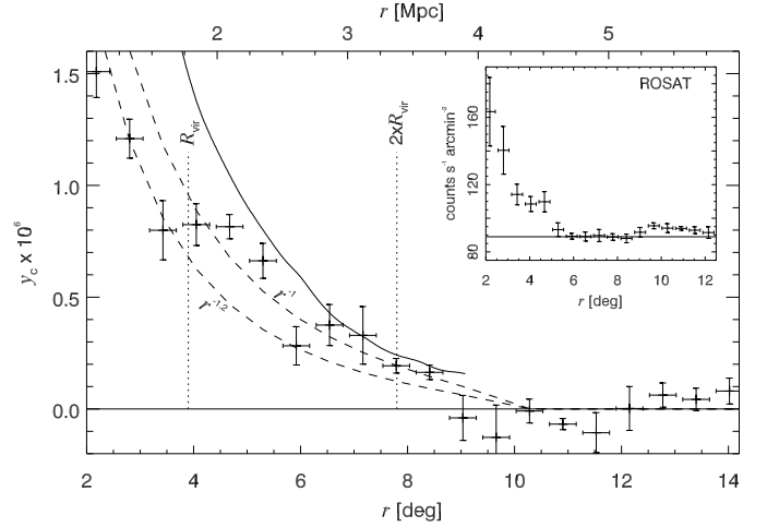
Fig. 15. Binned radial y_c profile of Virgo. The bins are 30 pixels wide (or equivalently 33' , or 230 \text{ kpc} ). The two dashed lines correspond to the expected signal from two analytical models where the electron density beyond 0.5 \text{ Mpc} falls as r^{-1} or r^{-1.2} . At r = 0.5 \text{ Mpc} the model is normalized to the electron density given by G04 at that distance. At distances smaller than 0.5 \text{ Mpc} the electron density follows the model of G04. The solid line shows the profile of the simulated Virgo cluster. The inset shows the corresponding profile in the ROSAT map using the same bins (with units the same as in Fig. 14)
