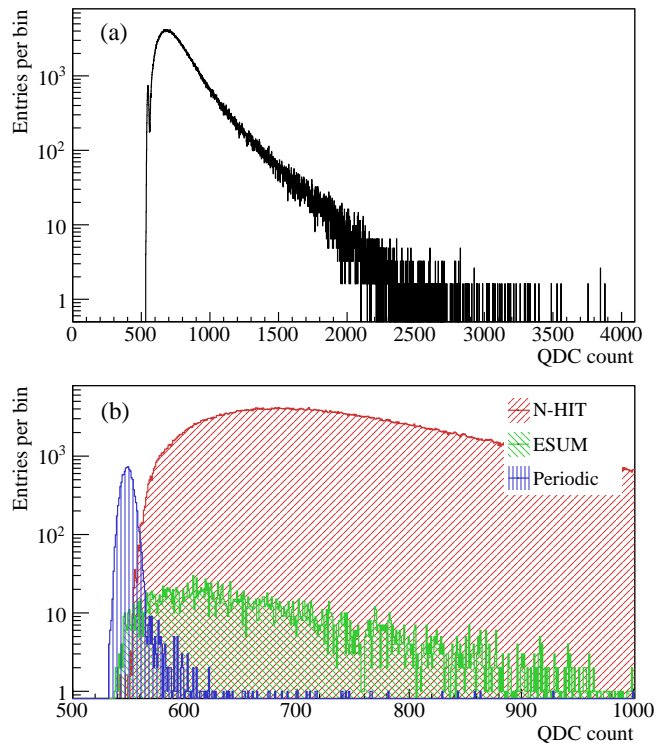
FIG. 6. (a) A typical charge histogram from the QDC output of a ND PMT regardless of the trigger type. (b) Charge histograms of different trigger types with the QDC count limited to 500–1000 to show the details at low energies.
