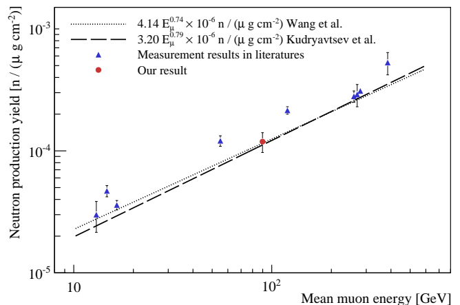
FIG. 17. Total neutron production yield as a function of muon energy. The dot represents our measurement result. The lines show the fitting result of FLUKA simulation studies [16, 27]. The triangles, from left to right, are other measurement results from, respectively, the Cosmic-ray Underground Background Experiment (CUBE) in the Stanford Underground Facility [3] (depth 20 m.w.e.), a gypsum mine [4] (depth 25 m.w.e.), the Palo Verde experiment [5] (depth 32 m.w.e.), a salt mine [4] (depth 316 m.w.e.), the Artemovsk Scientific Station [6] (depth 570 m.w.e.), the KamLAND experiment [7] (depth 2700 m.w.e.), the Large Volume Detector (LVD) in Gran Sasso [8] (depth 3650 m.w.e.), the Borexino experiment [9] (depth 3800 m.w.e.), and the Liquid Scintillation Detector (LSD) in Mont Blanc [10] (depth 5200 m.w.e.). For the measurement results, the abscissa corresponds to the average muon energy at the experimental depth.
