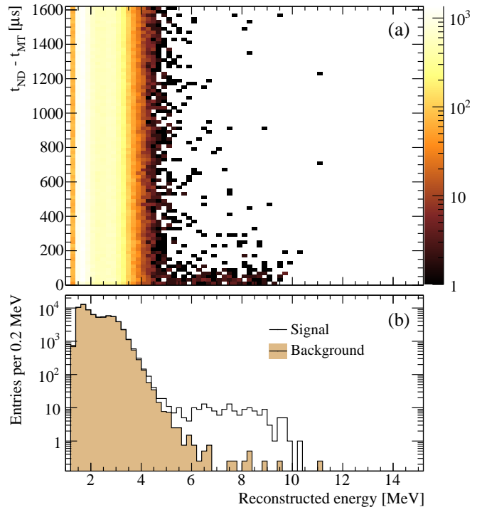
FIG. 16. (a) Energy and time distribution of ND signals following prompt MT signals. Muon-induced neutron-capture events can be seen around 8 MeV from 0 to 200 \mu s . (b) Comparison of ND energy spectra in the signal time window (10–210 \mu s ) and the background time window (800–1600 \mu s ). The background spectrum was scaled by a factor of 0.25.
