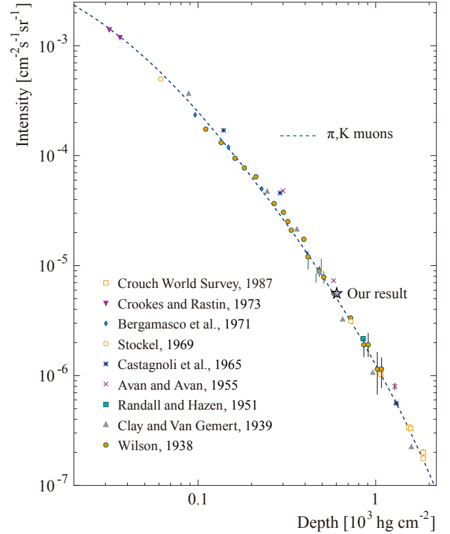
FIG. 13. Measured vertical muon flux as a function of depth, adopted from Ref. [20]. The current result is shown as a star, with error bars smaller than the size of the symbol.
