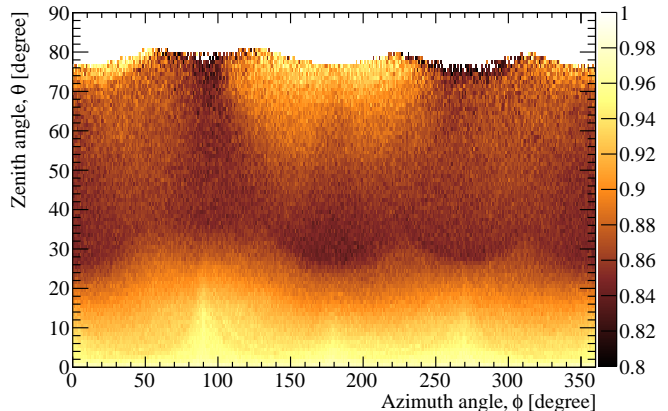
FIG. 8. Calculated efficiency of the MT with all the hodoscopes intact and under the trigger condition of 2/3-X and 2/3-Y. The maximum acceptance angle is about 80^\circ in zenith. The four tips correspond to the four corners of the MT.
