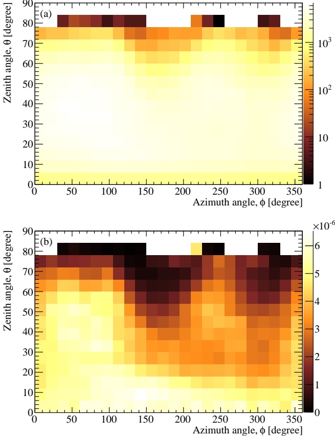
FIG. 12. (a) Measured number of muons and (b) muon intensity in the unit of \text{cm}^{-2}\text{s}^{-1}\text{sr}^{-1} . Both figures were drawn with a bin size of 6^\circ \times 15^\circ . The statistic uncertainty for each bin was in general better than 10%, except for \theta > 72^\circ where some bins had less than 100 events. The systematic uncertainty was about 10%.
