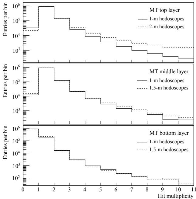
FIG. 5. Raw hit multiplicity of each MT hodoscope plane.
