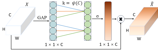
Figure 2: Diagram of the efficient channel attention (ECA) module. GAP stands for global average pooling.
