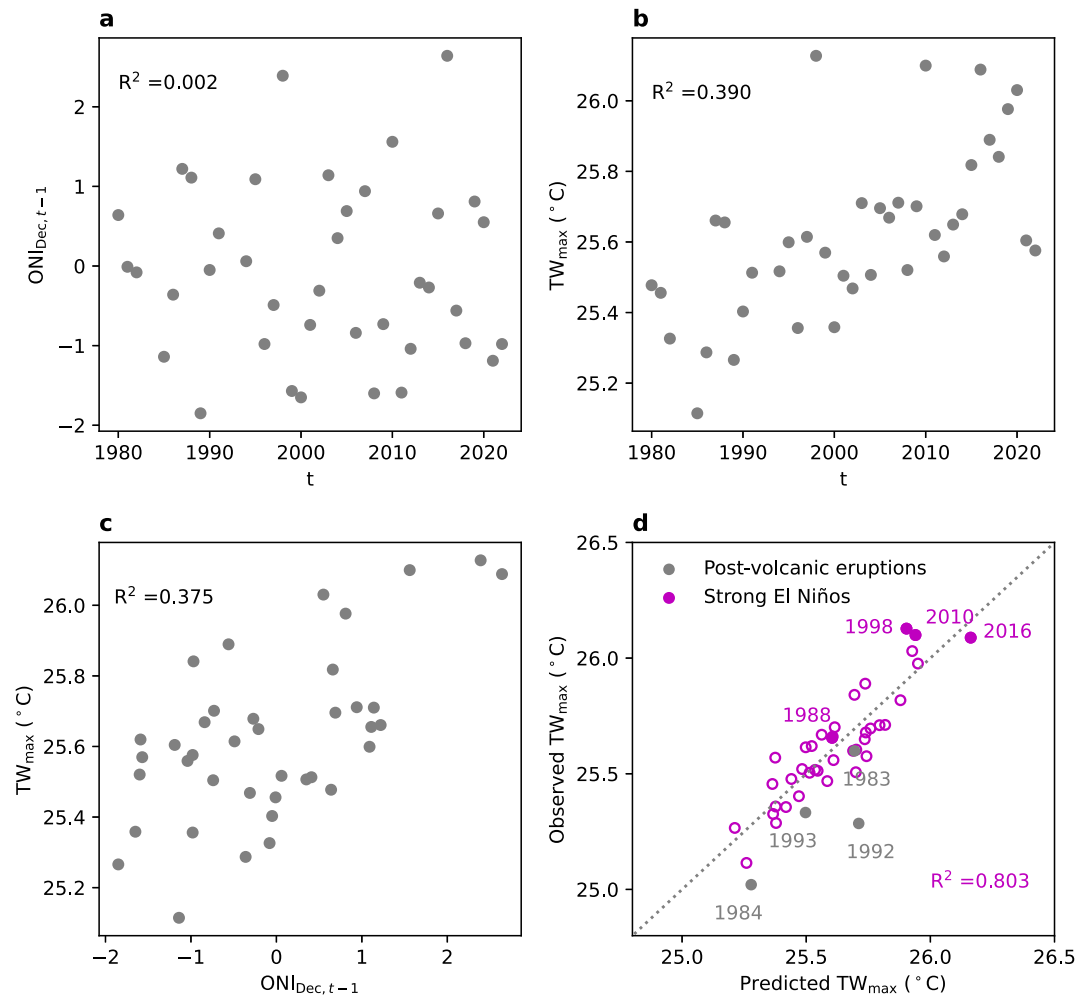
Figure 2. Visualization of the multiple linear regression for 30°S–30°N land-mean temperature ( TW_{max} ). a, Scatter plot of independent variables—December ONI of preceding years ( ONI_{Dec,t-1} ) and year ( t ). b, Scatter plot of 30°S–30°N land-mean TW_{max} and year ( t ). c, Scatter plot of 30°S–30°N land-mean TW_{max} and ONI_{Dec,t-1} . d, TW_{max} from ERA5 versus the predicted TW_{max} by the regression model. Years following major volcanic eruptions are excluded from the fit and are plotted separately in gray. Years after strong El Niños are highlighted. The gray dotted line indicates 1/1.
