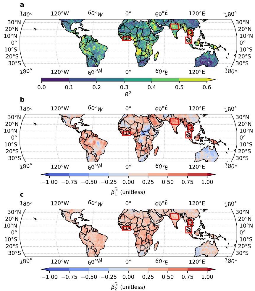
Figure 4. Results of fitting the model in Equation 4 at each location assuming generalized extreme value distributions of the error terms. a, R^2 , defined as the regression sum of squares divided by the total sum of squares. Red boxes outline regions of interest further analyzed in Figure 5 b, Standardized regression coefficient of warming. c, Standardized regression coefficient of El Niño-Southern Oscillation variability.
