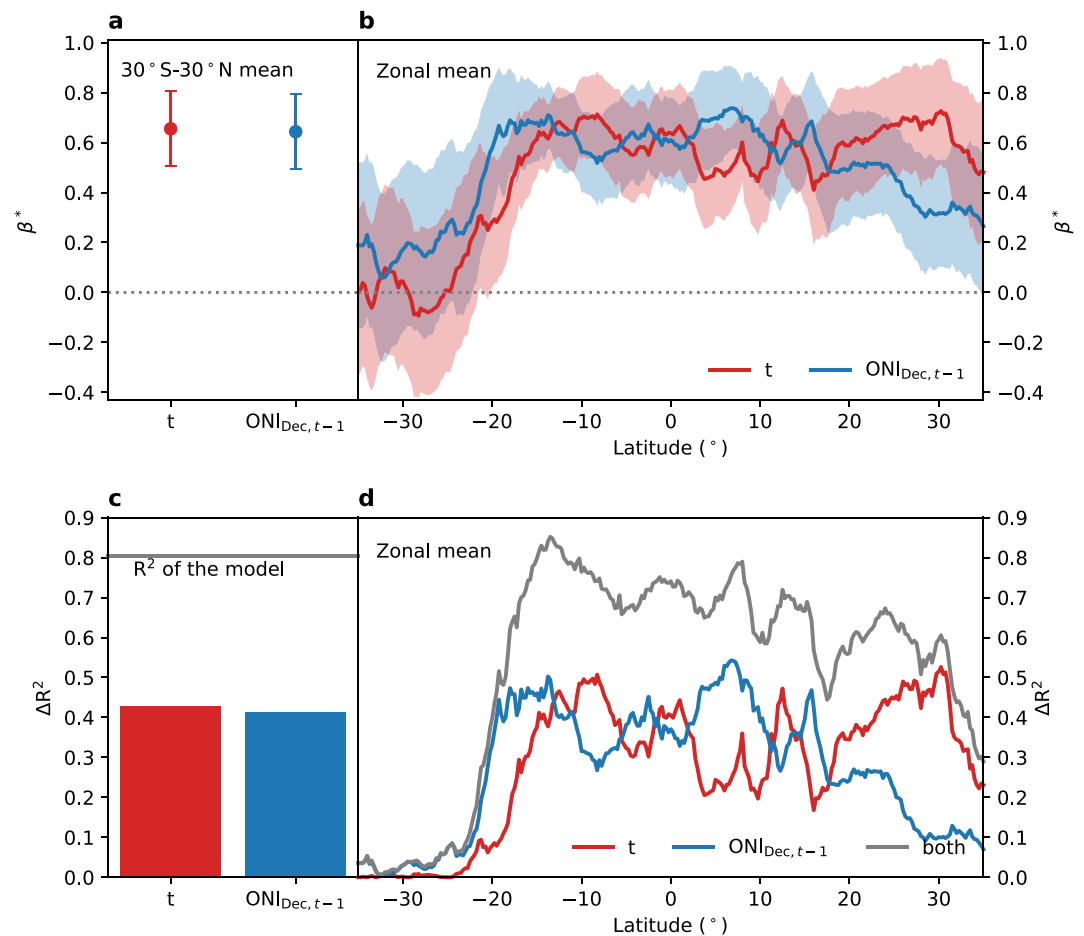
Figure 3. Relative importance of constant warming and El Niño-Southern Oscillation variability in explaining temperature ( TW_{max} ) variability. a, Standardized regression coefficients ( \hat{\beta}^* ) and the 95% confidence intervals for both independent variables. b, Same as a but for zonal mean TW_{max} over land. c and d, Incremental R^2 ( \Delta R^2 ) for each independent variable, estimated by removing each variable from the full regression, and the R^2 of the full model (gray).
