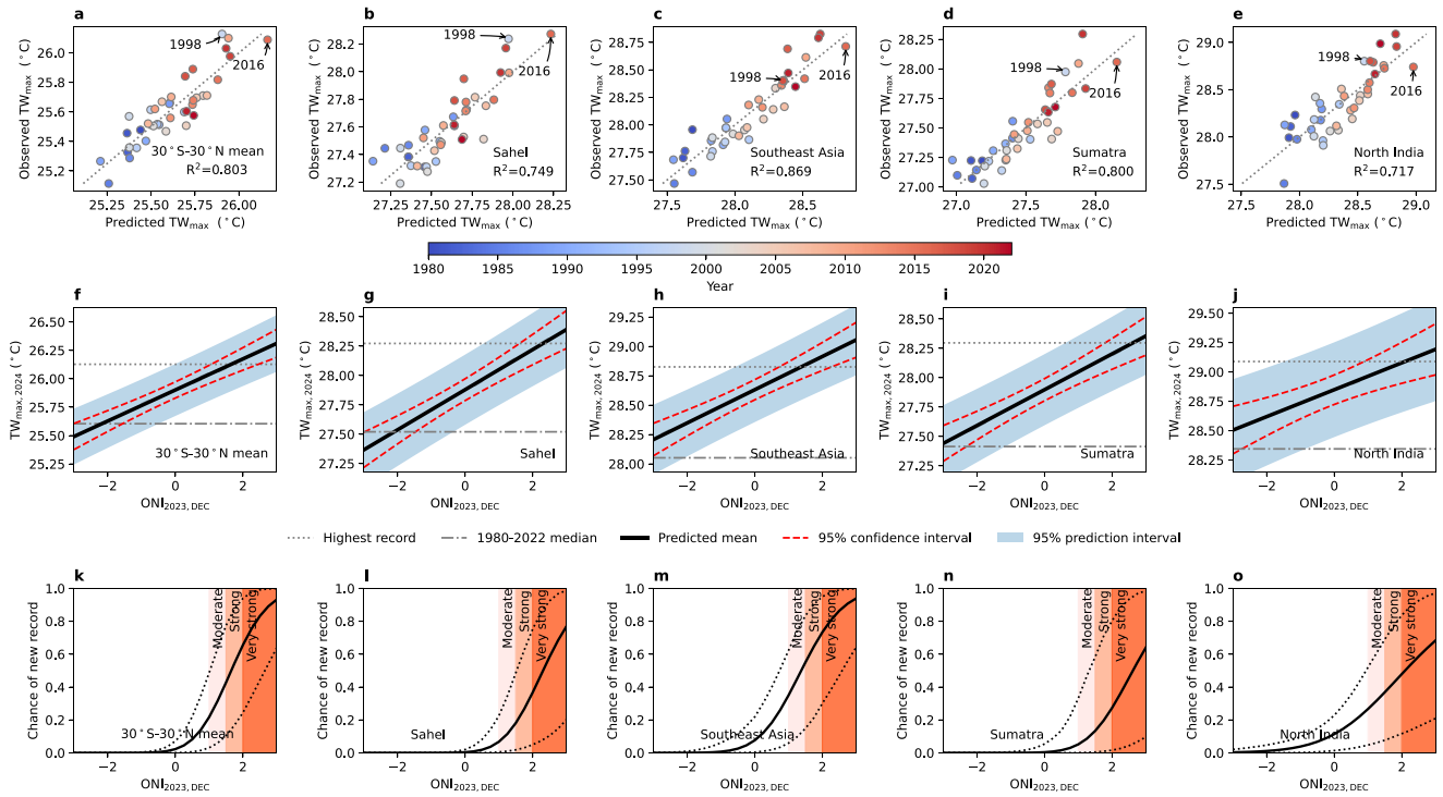
Figure 5. Example temperature ( TW_{max} ) forecast for 2024. a-e, Performance of multiple linear regression for 30°S–30°N land mean and four regions marked in Figure 4a. Color indicates the year of the data point. Two major El Niños-1998 and 2016-are highlighted. f-j, Predicted TW_{max, 2024} as a function of December Oceanic Niño Index (ONI), 2023. Confidence intervals in red account for the standard error of the predicted mean. Prediction intervals in blue additionally take into account the year-to-year variability around the predicted mean. k-o, Estimated chance of TW_{max} setting new records in 2024 in the tropical mean and each region conditioned upon the strength of El Niño by the end of 2023. ONI ranges of moderate ( 1.0 \leq ONI < 1.5 ), strong ( 1.5 \leq ONI < 2.0 ) and very strong ( ONI \geq 2.0 ) El Niño events are marked.
