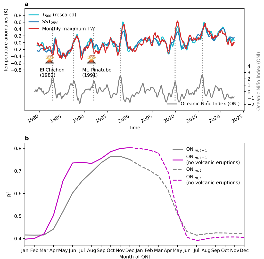
Figure 1. El Niño-Southern Oscillation variability leads tropical land TW_{max} by a few months. a, Monthly anomalies of tropical (between 30°S and 30°N) land mean TW_{max} (red), the upper-quartile-mean sea surface temperature (blue) from Hadley Center Sea Ice and SST data set (Rayner et al., 2003), and the average 500-hPa temperature divided by the moist adiabatic amplification factor 1.4 (cyan), as well as the Oceanic Niño Index (ONI) in gray. Timing of strong El Niños (ONI > 1.5) are marked with vertical dotted lines. b, R^2 values of the multiple linear regression model specified in Equation 4 using ONI from January to December of preceding years (solid) and contemporaneous years (dashed). The gray line shows the fit using all 43 years between 1990 and 2022, while the magenta line shows the fit of 39 years to exclude major volcanic eruptions.
