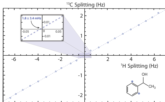
FIG. 5. Experimental data showing the diastereomeric splitting of the ^{13}\text{C} peaks vs the diastereomeric splitting of the ^1\text{H} peaks as the chirality of the solvent is titrated. A nonzero intercept on the vertical axis would be an indication of PNC effects.
