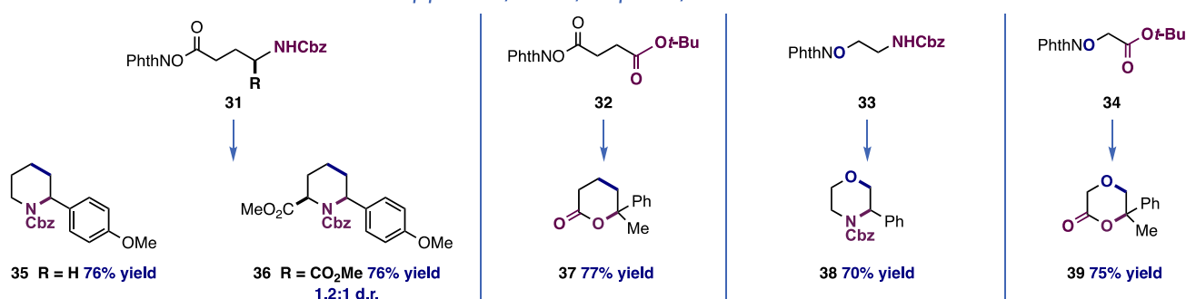
Figure 2. Substrate scope of [3 + 2] and [4 + 2] annulation reactions. Reactions run on 0.5 mmol scale unless otherwise noted. Yields are for isolated material and are the average of two runs. All products generated from achiral starting materials are racemic. a Gram-scale reaction performed using 0.2 mol % photocatalyst with 24 h. reaction time. b Reaction performed on 0.1 mmol scale. c Gram-scale reaction performed using 0.5 mol % photocatalyst. See the Supporting Information for details on relative stoichiometries of reagents.
