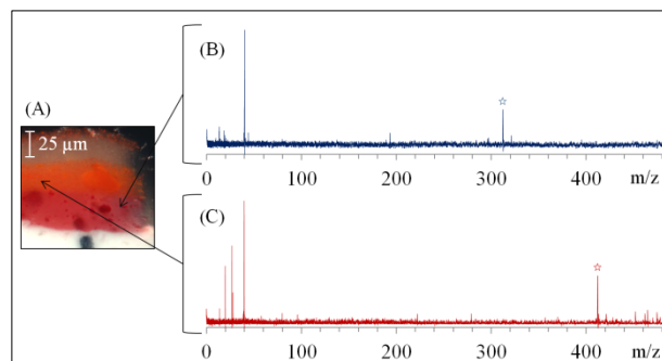
Fig 5: (A) Microscope image of synthetic dye cross section. The sequence of layers from bottom to top: PV19, PO43, PY151 and PR254. (B) Mass spectrum (non-resonant) obtained from PV19 dye layer and (C) non-resonant ionization mass spectrum (non-resonant) from PO43 dye layer. Stars denote parent mass peaks.
