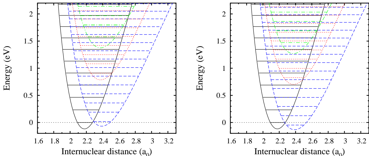
FIG. 1: (Color online) NO and NO - potential curves and vibrational levels. Solid curves: 2 Π neutral ground-state; dashed curves: 3 Σ - anion; dotted curves: 1 Δ anion; dash-dot curves: 1 Σ + anion. Left panel: curves obtained from configuration-interaction calculations; right panel: shifted CI curves (see text). Internuclear distances are given in atomic units, where a_0 = 5.2917721 \times 10^{-11} m is the Bohr radius. Energies are in units of eV = 1.6021765 \times 10^{-19} J.
