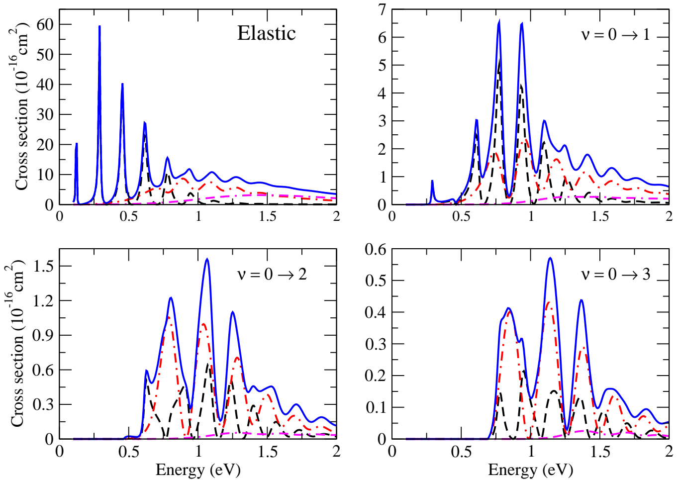
FIG. 3: (Color online) Contribution of individual resonances to the elastic and vibrationally inelastic cross sections. Solid curves: total cross sections; dashed curves: {}^3\Sigma^- symmetry contributions; dash-dot curves: {}^1\Delta symmetry contributions; double dash-dot curves: {}^1\Sigma^+ symmetry contributions. Individual symmetry contributions include statistical weights given in Eq. (15).
