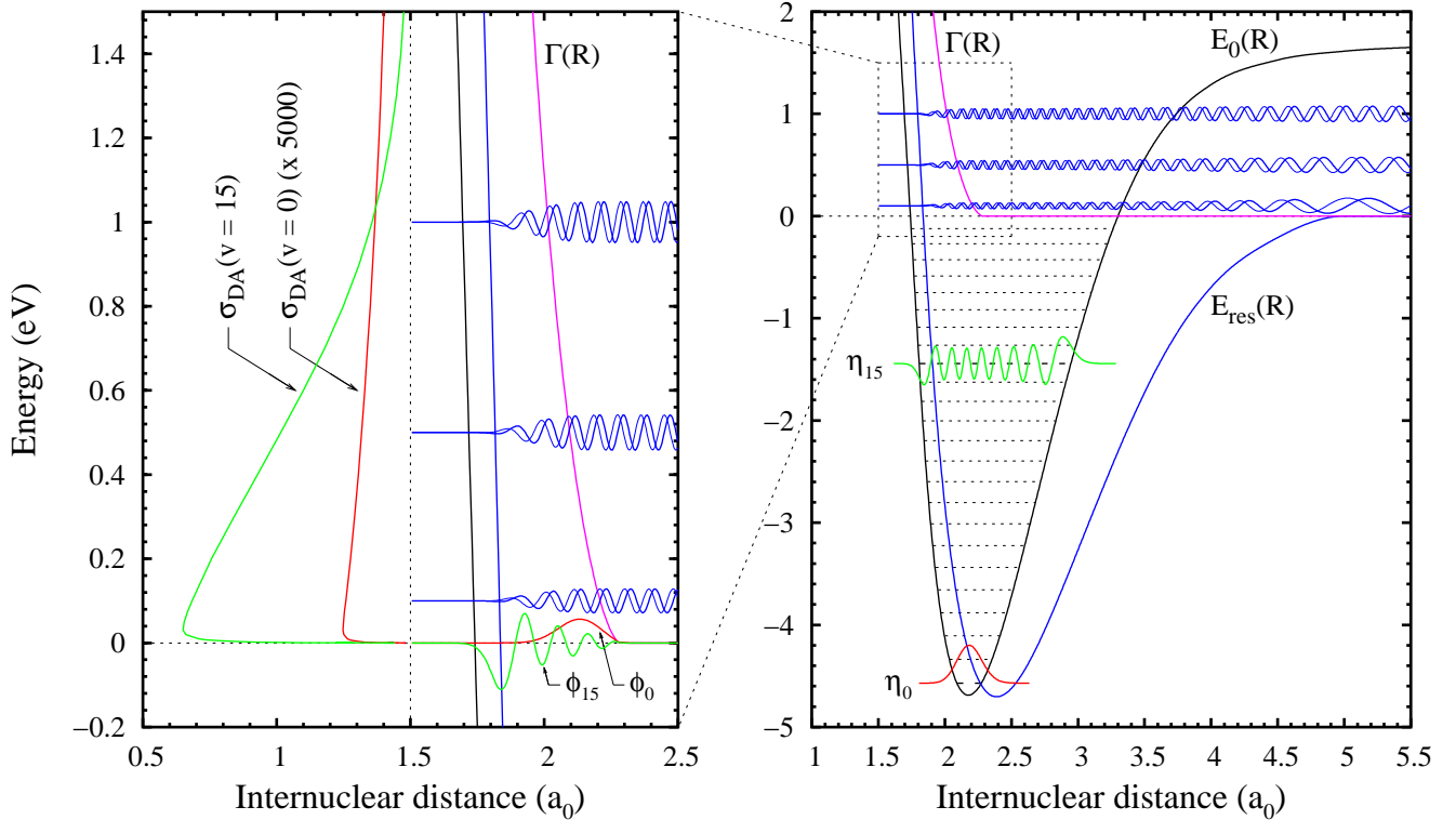
FIG. 8: (Color online) Right panel: Potential energy curves of NO and of the {}^3\Sigma^- resonance (solid curves), and vibrational levels of the neutral target (dotted lines). Also shown are the vibrational wave functions \eta_0(R) and \eta_{15}(R) and the scattering solution of Eq. (22), \psi_E , at E = 0.1, 0.5 and 1.0 eV (solid curves). Left panel: enlargement of the selected region of the right panel. In addition to the wave functions mentioned above, the entry amplitudes \phi_0(R) and \phi_{15}(R) (see Eq. (6)) are shown. Vibrationally excited DA cross sections are plotted for \nu = 0 ( \sigma_{DA}(\nu = 0) \times 5000 ), and for \nu = 15 ( \sigma_{DA}(\nu = 15) ). Internuclear distances are given in atomic units and energy in units of eV.
