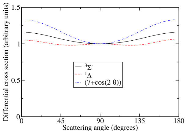
FIG. 5: (Color online) Angular dependence of resonant cross sections. With the assumption of a single partial wave, the resulting distribution is (7 + \cos 2\theta) for both {}^3\Sigma^- and {}^1\Delta cross sections. The angular distributions for {}^3\Sigma^- and {}^1\Delta are different when more partial waves are used in the analysis (see text).
