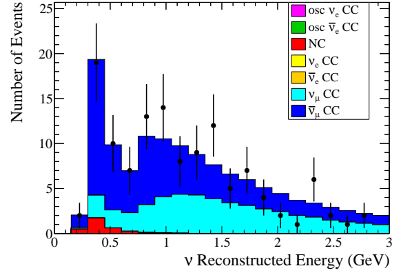
(b) RHC 1-Ring \mu -like
