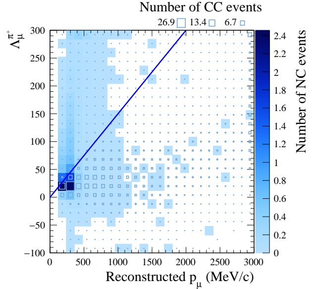
FIG. 28: The width of \sin^2 \theta_{23} 1\sigma confidence interval as a function of the slope and intercept of the \text{NC}\pi^+ rejection cut line is shown on the top and the distribution of signal and background events is shown on the bottom, along with the line below which \mu -like events are selected.
