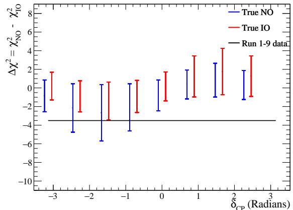
FIG. 70: Ability to distinguish between the two mass orderings as a function of the true value of \delta_{\text{CP}} . The bar indicates the range of values of \Delta\chi^2 = \chi_{\text{NO}}^2 - \chi_{\text{IO}}^2 which contains 95% of the values obtained for the pseudo-experiments generated in each case. The black line corresponds to the value obtained in the data fit by Analysis A.
