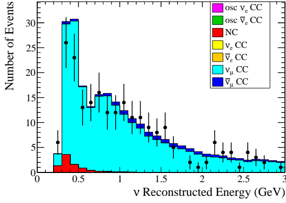
(a) FHC 1-Ring \mu -like
