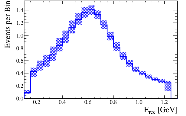
FIG. 42: Post-ND280-fit predicted event spectrum for the RHC SK samples as a function of E_{\text{QE}}^{\text{Rec}} . The samples are: single-ring muon-like (top) and single-ring electron-like without decay electrons (bottom).
