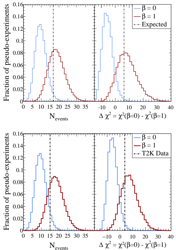
FIG. 73: Distributions of the expected (top) and observed (bottom) rate-only (left) and rate+shape (right) test statistics compared to the expected/observed test statistics. Here N_{\text{events}} denotes the number of observed events in the RHC single-ring e -like sample.
