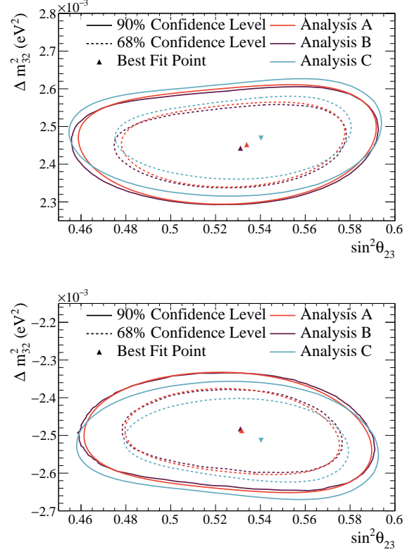
FIG. 58: Comparison between the observed 1\sigma (dashed) and 90% (solid) CL regions for \Delta m^2 vs \sin^2\theta_{23} produced using analyses A, B and C, assuming normal mass ordering (top) or inverted mass ordering (bottom). The reactor constraint is applied.
