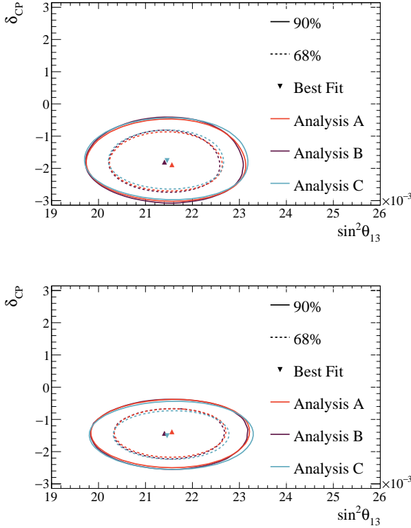
FIG. 57: Comparison between the observed 1\sigma (dashed) and 90% (solid) CL regions for \delta_{CP} vs \sin^2\theta_{13} produced using analyses A, B and C, assuming normal mass ordering (top) or inverted mass ordering (bottom). The reactor constraint is applied.
