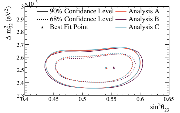
FIG. 47: Comparison between analyses A, B and C. The normal mass ordering is assumed and the reactor constraint is applied. Top: the predicted \Delta\chi^2 functions for \delta_{CP} . Bottom: the 1\sigma (dashed) and 90\% (solid) CL regions for \Delta m^2 vs. \sin^2 \theta_{23} .
