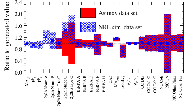
FIG. 50: Results of the fit to the near detector simulated data with an increased nucleon removal energy. The best fit values for the \nu_\mu flux parameters at SK (top) and cross-section parameters (bottom) are shown for the NRE fit (blue) compared to the Asimov data set fit (red).
