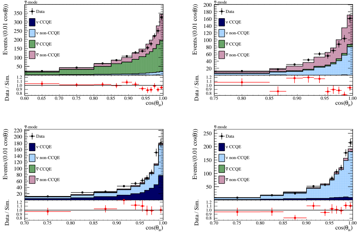
FIG. 14: Distributions of the final state muon angle for the RHC \bar{\nu}_\mu (top) and \nu_\mu (bottom) CC 1-track (left) and CC N -track (right) FGD1 simulation samples. These distributions are before the ND280 fit.
