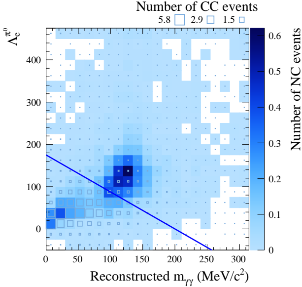
FIG. 29: The sensitivity to exclude \delta_{\text{CP}} = 0 as a function of the slope and intercept of the \text{NC}\pi^0 rejection cut line is shown on the top and the distribution of signal and background events is shown on the bottom, along with the line below which e -like events are selected.
