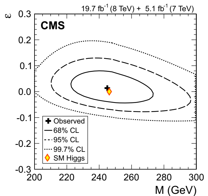
lihood scan for the M and \epsilon parameters of the model detailed in the text. The cross indicates the best-fit values. The solid, dashed, and dotted contours show the 68 %, 95 %, and 99.7 % CL confidence regions, respectively. The diamond represents the SM expectation, (M, \epsilon) = (v, 0) , where v is the SM Higgs vacuum expectation value, v = 246.22 GeV
