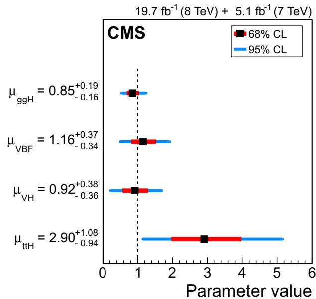
Fig. 6 Likelihood scan results for \mu_{ggH}, \mu_{VBF}, \mu_{VH}, and \mu_{ttH} . The inner bars represent the 68 % CL confidence intervals while the outer bars represent the 95 % CL confidence intervals. When scanning each individual parameter, the three other parameters are profiled. The SM values of the relative branching fractions are assumed for the different decay modes
