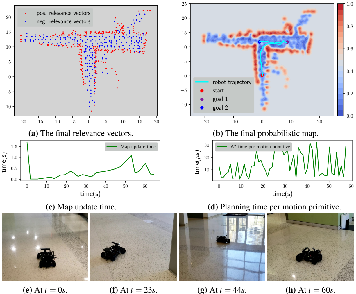
Figure 5.10. Real experiment with an autonomous Racecar robot navigating in an unknown hallway environment.
