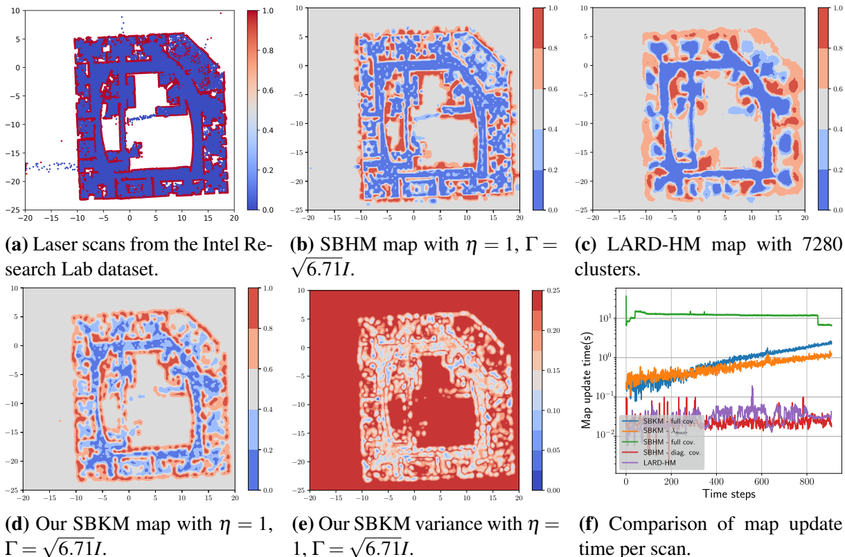
Figure 3.4. Comparison among sparse Bayesian kernel-based map (SBKM), LARD-HM [56], and SBHM [148] on the Intel Research Lab dataset [70].
