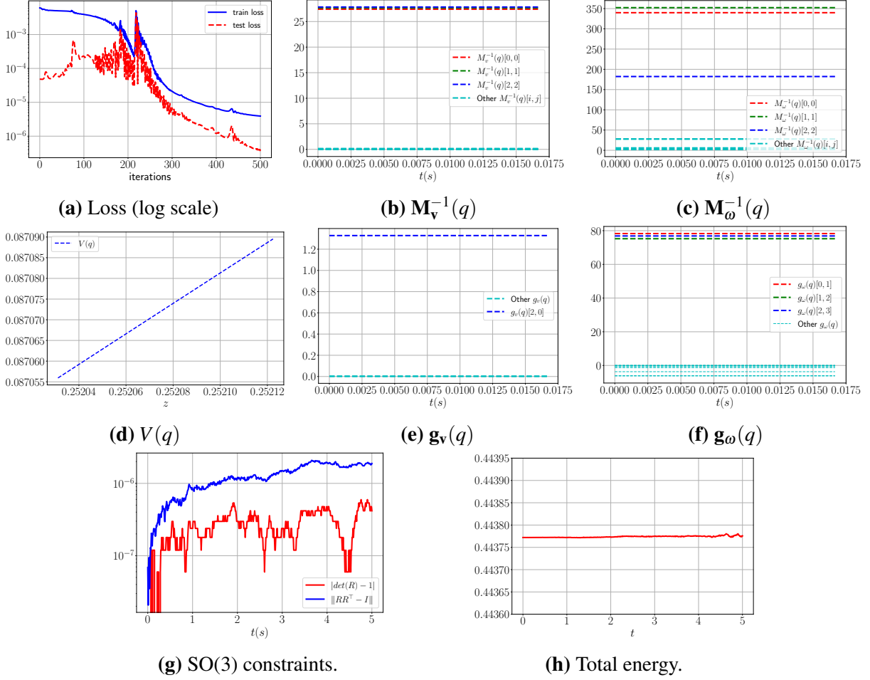
Figure 4.4. Evaluation of the SE(3) Hamiltonian neural ODE network on an under-actuated Crazyflie quadrotor in the PyBullet simulator [129].
