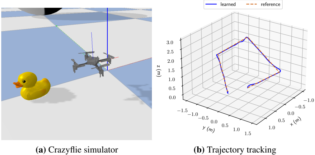
Figure 5.6. Trajectory tracking experiment with a Crazyflie quadrotor in the PyBullet simulator [129].
