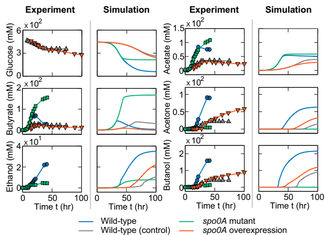
Fig. 5. Comparison of the computational and experimental fermentation profiles for the strains with genetic network perturbations. The fermentations of the spo0A -knockout (green lines), spo0A overexpression (red lines), and their control (blue and gray lines) strains were simulated with the integrated model and further compared with corresponding experimental results reported in previous studies [green squares (33), red triangles (34), blue circles (33), and gray triangles (34)]. Notice that the experimental data do not include the glucose consumptions of the WT and spo0A -mutant strains and the ethanol yields for the spo0A overexpression strain and its control, due to the lack of information in the original literature.
