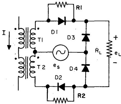
Fig. 5 - Parallel Transducer
