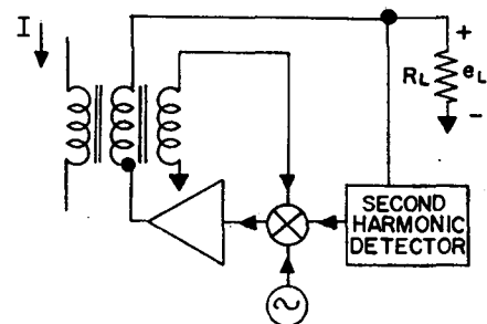
Fig. 10 - Feedback Transducer
