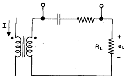
Fig. 9 - Additional Core Filter (replaces $R_L$)
