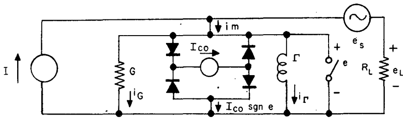
Fig. 3 - Single Core Transducer with Core Model
