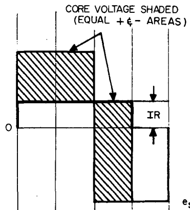
Fig. 2 - Single Core Transducer Waveshapes
