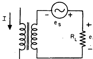
Fig. 1 - Single Core Transducer
