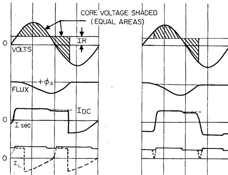
Fig. 7 - Parallel Transducer Waveshapes
