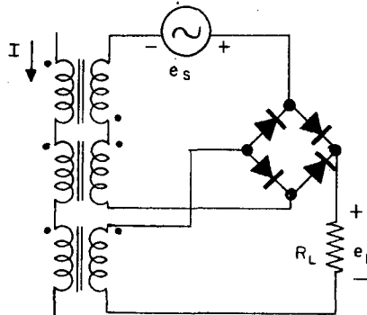
Fig. 6 - Series Transducer
