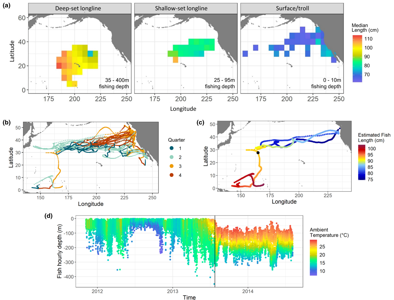
FIGURE 3 (a) Spatial distribution of median length of albacore landed with deep-set longline, shallow-set longline, and troll (i.e., surface) fishing gear. Lengths of fish caught by surface gear are sampled at US and Canadian ports when fish are landed (Childers, 2001), whereas lengths from longline catches are recorded by fisheries observers. Longline gear depths are from Bigelow et al. (2006) and Woodworth-Jefcoats et al. (2018). (b) Daily locations (color-coded by season) of 25 albacore tagged with archival tags. (c) Daily locations for a tagged albacore released as a 74.5 cm juvenile on October 8th, 2011 and recaptured as a 103 cm adult on August 7th, 2014. (d) Hourly fish depth and ambient temperature for the same fish, showing estimated length. The approximate date of transition from surface-based juvenile behavior to subsurface adult behavior is indicated by the black dot in (c) and the black vertical line in (d).
