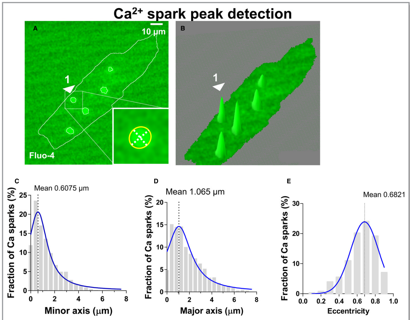
Figure 3. Ca 2+ spark peak detection. A, Representative confocal Fluo-4 fluorescence frame extracted from 600 sequential frames. White outline indicates cell border, and yellow outlines indicate sparks detected for this frame (inset shows enlargement of region 1) with major and minor axes depicted. B, 3-Dimensional surface plot of the same frame as in A with the signal over the spark threshold detection shown. The threshold is set at 1 standard deviation above the local mean intensity. C and D, Distribution of Ca 2+ spark major axis and minor axis lengths (N=8 cells, n=1 rat, Lorentzian fit). E, Distribution of spark shape eccentricity (see also RyR cluster eccentricity in Figure S5, Gaussian fit). RyR indicates ryanodine receptors.
