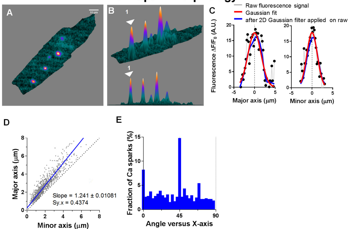
Figure S6. Refinement of Ca 2+ spark Morphology. (A-B) Peak amplitude and mean intensity were used to reduce false-positive events and obtain clear Ca 2+ spark profiles, viewed in the x-y plane (A) and from an oblique and side angle (showing intensity in both color and height). (C) Spatial profiles for raw \Delta F/F_0 (gray) and after applying a simple Gaussian fit on the raw profile (red) or after applying a 2D Gaussian filter (blue). This method provides accurate localization of Ca 2+ spark peaks. (D) The shape of Ca 2+ sparks. Major axis vs Minor axis. The slope was 1.24 \pm 0.01 , which indicates slightly ellipsoidal (n=4 cells, N=1 rat, Linear regression fit). (E) Distribution of Ca 2+ spark orientation. This graph shows that there is no preferred orientation.
