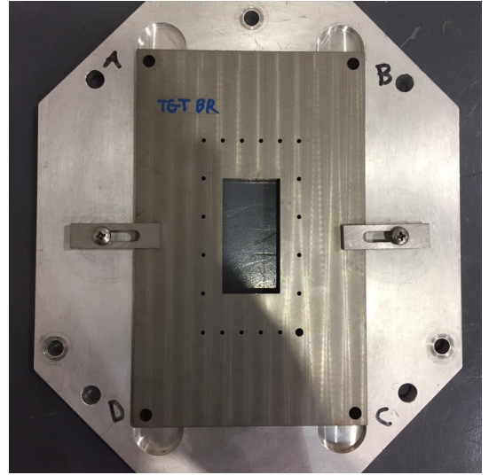
Fig. 2. Photo of the tungsten (grey) 2 mrs collimator with its outer sieve holes that was used during the LEDEX experiment. The outer aluminum frame mounted to the face of the HRS spectrometer with mounting bolts located at A,B,C and D. The tungsten plate could be removed if full HRS acceptance was desired without removing the outer aluminum frame. Sieve photo courtesy of Jessie Butler.
