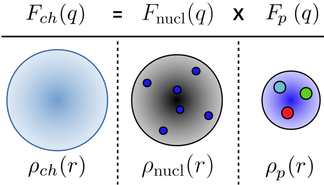
Fig. 8. Relationship between the charge, nucleons (protons) and the single proton form factors along with their respective densities for ^{12}\text{C} . The protons density \rho_{nucl} specifies the spatial distribution of the 6 protons inside the ^{12}\text{C} nucleus, treating them as point particles (blue circles over the black background in the middle column). The charge form factor F_{ch} , which relates to the charge distribution in the nucleus (left column), is the result of folding the protons form factor F_{nucl} with the single proton form factor F_p , which relates to the charge distribution inside the proton (right column, the color circles represents the three quarks).
