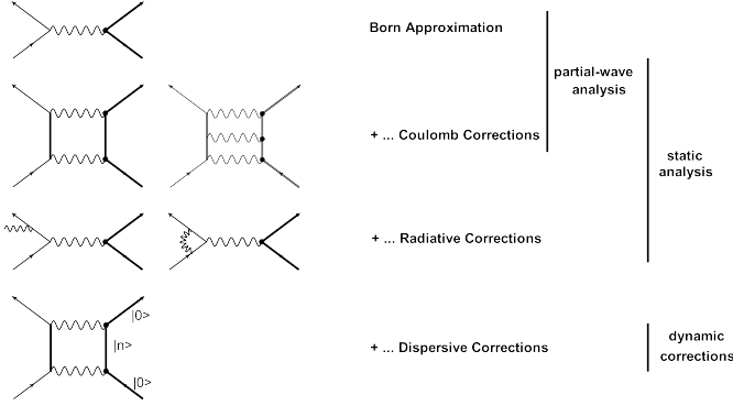
Fig. 1. High-order corrections to the one-photon exchange Born approximation in electron/positron-nucleus scattering.
