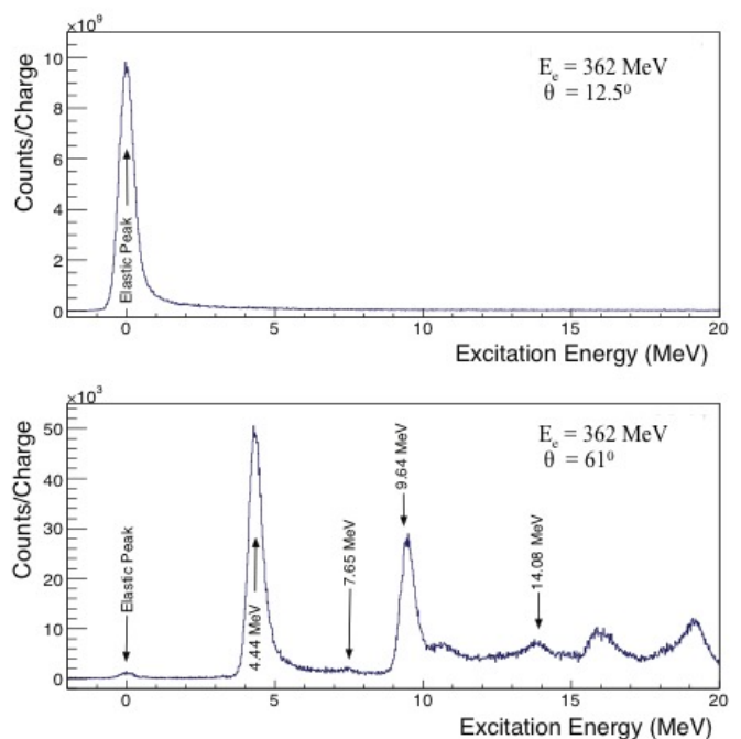
Fig. 4. The reconstructed excitation energy distributions at E_c = 362 MeV for \theta = 12.5^\circ (top) and \theta = 61^\circ (bottom) scattering angles.
