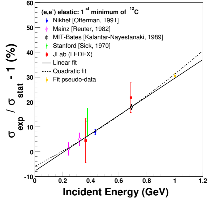
Fig. 6. World data on the energy dependence of dispersive effects in the first diffraction minimum of 12 C. In the y-axis, \sigma_{stat}^{FB} was replaced by \sigma_{stat} to keep coherency in the text. The first minimum at q_{eff} = 1.84 fm -1 moves slightly with beam energy as noted in [37] (this dependency is out of the scope of this paper).
