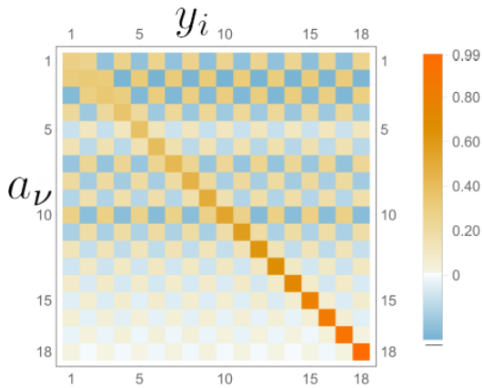
Fig. 9. \partial a_\nu/\partial y_i matrix for the data extracted from Offermann et al. [4].
