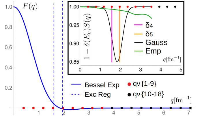
Fig. 10. ^{12}\text{C} form factor expanded in the Bessel functions using Offermann [4] coefficients without dispersive corrections. The circles in the q axis shows the special values of momentum transfer for the first 9 (red) from experimental data and the second 9 (black) from the extrapolation suggested in [43]. The dashed blue lines encloses the region of the data excluded from the analysis in [4]. The inset plot shows the three test forms for S(q) in addition to the empirical perturbation obtained directly from the data by third degree spline interpolation. The curves in the inset plot are the ones needed to obtain the corrected F_{\text{ch}}^{\text{stat}} from the observed F_{\text{ch}}^{\text{disp}} values.
