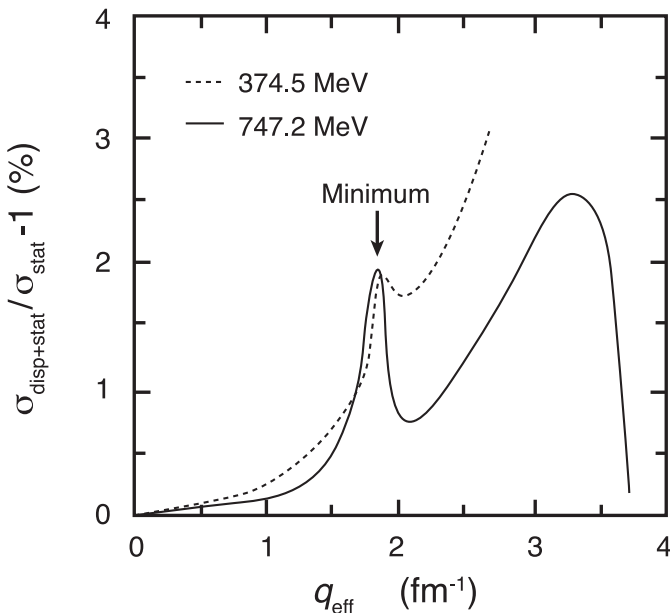
Fig. 7. Calculations of Friar and Rosen [24] for dispersion corrections to elastic electron scattering from ^{12}\text{C} at 374.5 and 747.2 MeV in the first diffraction minimum q_{eff} = 1.84 \text{ fm}^{-1} .
