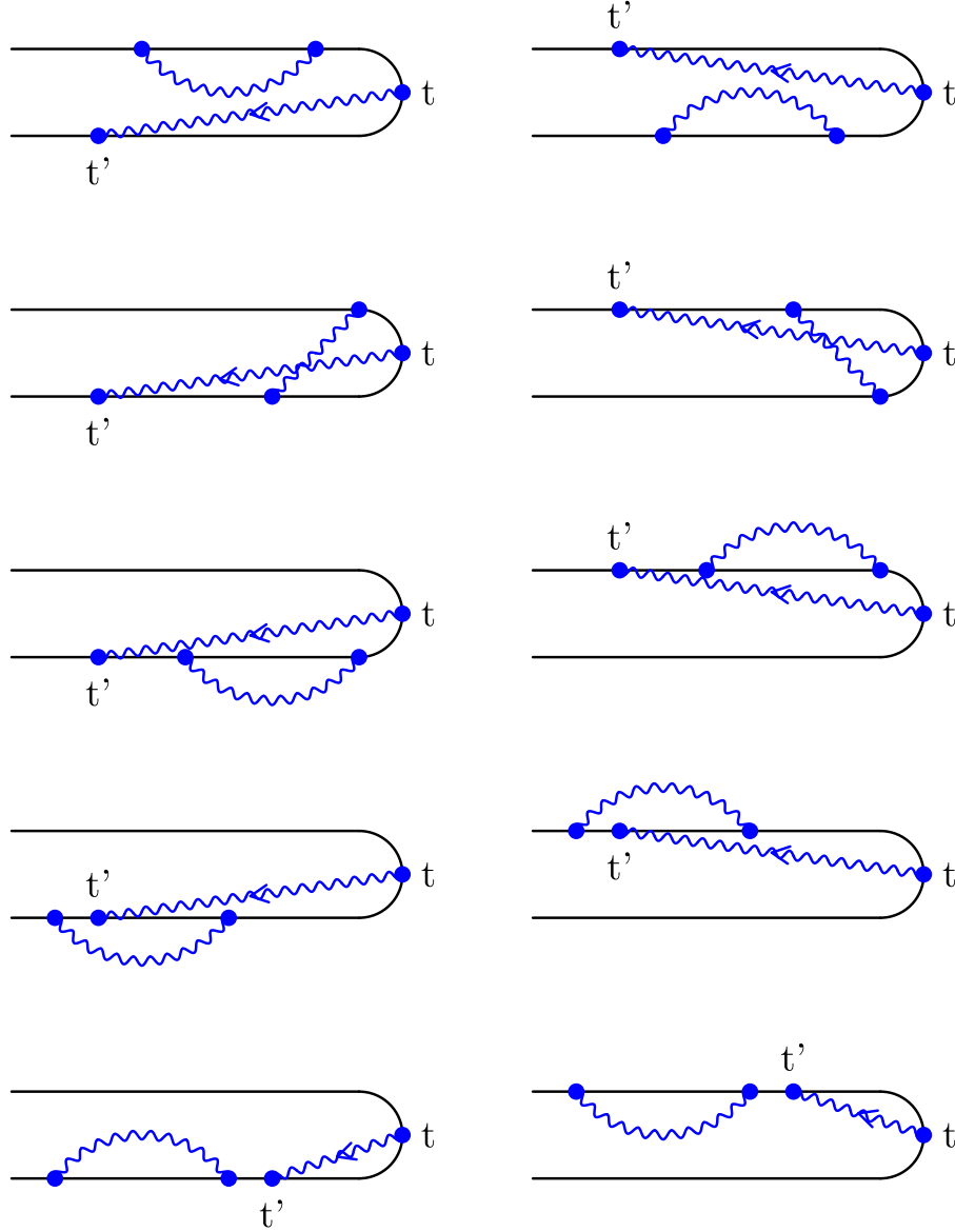
Figure 4: Double-sided Feynman diagrams for fourth order optical processes in the photon flux. Wavy line (blue) is the photon Green's function F , eq 14. Left (right) column corresponds to first (second) term in the right side of eq 26. Wavy line without arrow stands for F(\tau_3, \tau_4) of eq S2. Both arrow directions are possible in this line.
