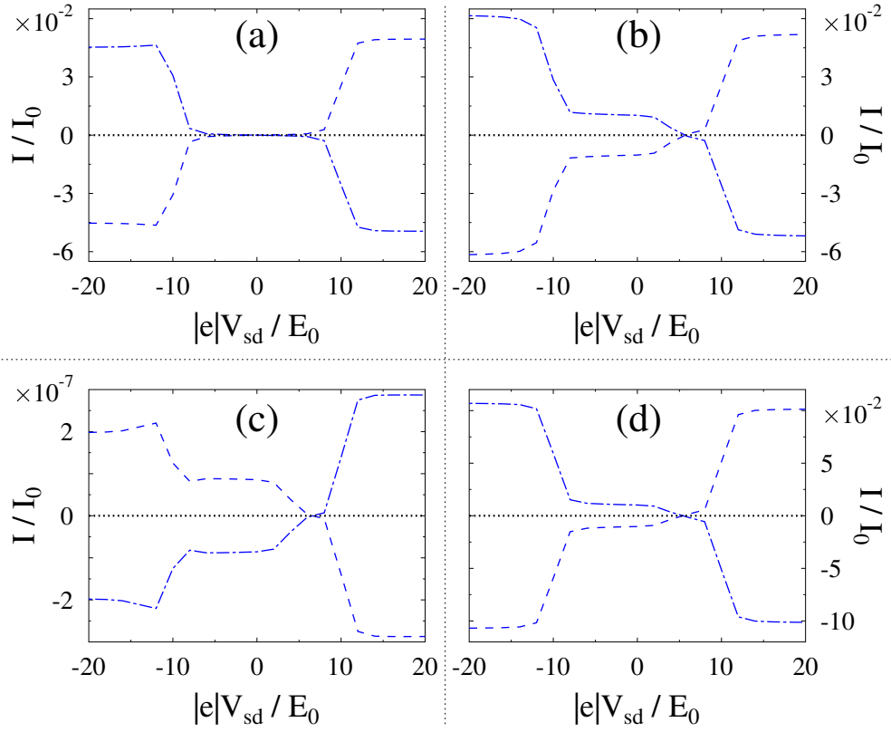
Figure 6: Charge conservation, eq 34, for the junction model of Figure 5. Shown are I_L (dashed line, blue), I_R (dash-dotted line, blue) and their sum (dotted line, black) for (a) zero, (b) second, and (c) fourth order contributions; (d) shows total fluxes, eq 36. See text for parameters.
