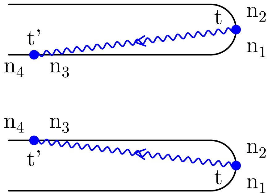
Figure 3: Double-sided Feynman diagrams for second order optical processes in the photon flux, eq 29. Wavy line (blue) is the photon Green function F , eq 14. Top (bottom) diagram corresponds to first (second) term in the right side of eq 29. Indices n_i indicate molecular orbitals.
