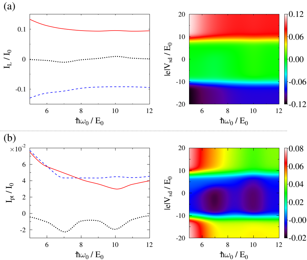
Figure 8: Particle fluxes vs. pumping frequency \omega_0 for the junction model of Figure 5. Shown are (a) I_L = -I_R , eq 36, and (b) I_{pt} , eq 37, at biases |e|V_{sd} = -16 E_0 (dashed line, blue), |e|V_{sd} = 0 (dotted line, black), and |e|V_{sd} = 16 E_0 (solid line, red) in left panels. Right column shows map of the fluxes vs. pumping frequency \omega_0 and bias V_{sd} . See text for parameters.
