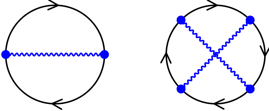
Figure 1: Diagrammatic perturbation theory within NEGF. Shown are the Luttinger-Ward generating functionals for second (left) and fourth (right) order expansion in light-matter interaction. Directed solid line (black) represents the electron Green function G , eq 13. Wavy line (blue) is the photon Green function F , eq 14; both directions are implied here. Solid circles indicate vertices. Summation over all degrees of freedom and integration over contour variables is assumed at the vertices.
