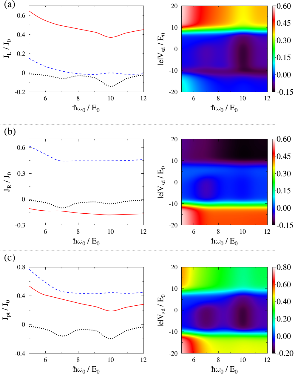
Figure 9: Energy fluxes vs. pumping frequency \omega_0 for the junction model of Figure 5. Shown are (a) J_L , eq 38, (b) J_R , eq 38, and (c) J_{pt} , eq 39, at biases |e|V_{sd} = -16 E_0 (dashed line, blue), |e|V_{sd} = 0 (dotted line, black), and |e|V_{sd} = 16 E_0 (solid line, red) in left panels. Right column shows map of the fluxes vs. pumping frequency \omega_0 and bias V_{sd} . See text for parameters.
