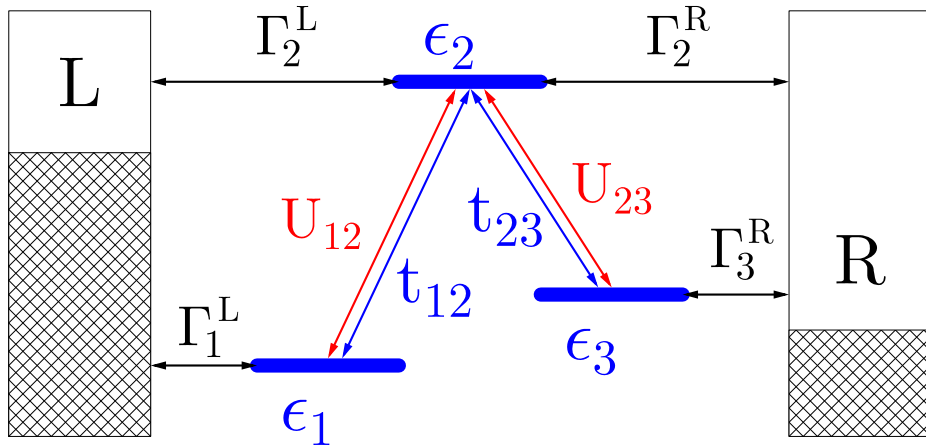
Figure 5: Donor (1) - bridge (2) - acceptor (3) junction model for photo-assisted electron transport.
