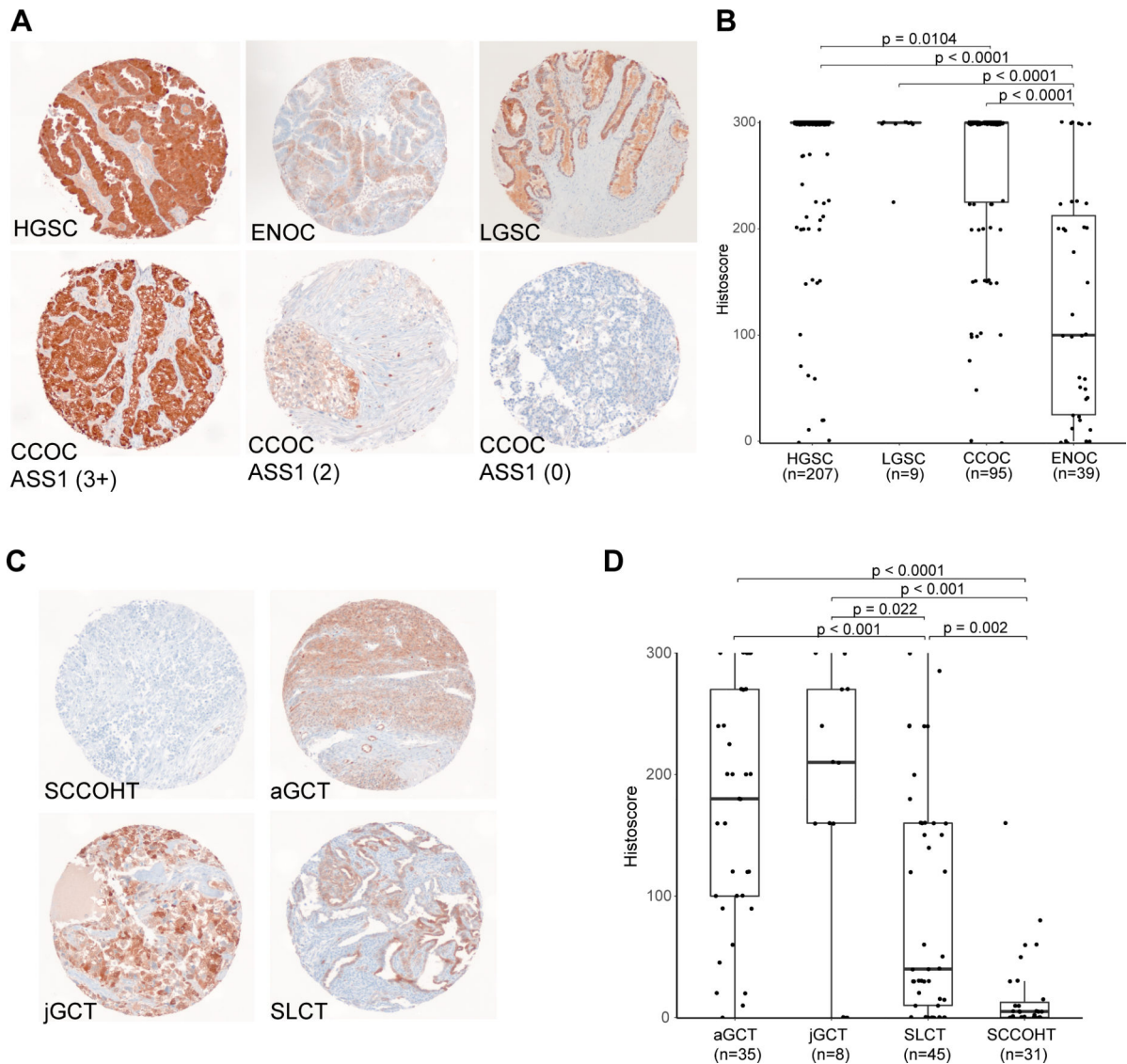
Figure 2. ASS1 immunohistochemistry demonstrates differential expression in ovarian cancer subtypes.
