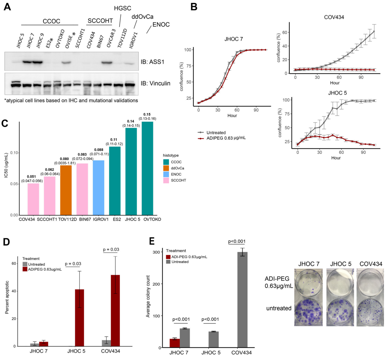
Figure 3. ASS1 deficient ovarian cancer are sensitive to arginine deprivation through ADI-PEG20.
