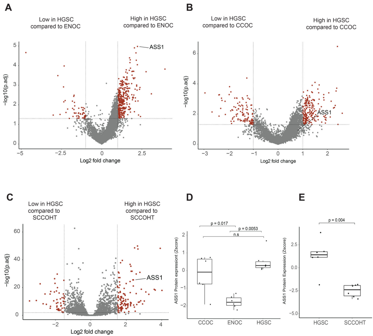
Figure 1. Global proteomics identifies decreased ASS1 expression in rare ovarian cancer subtypes.
