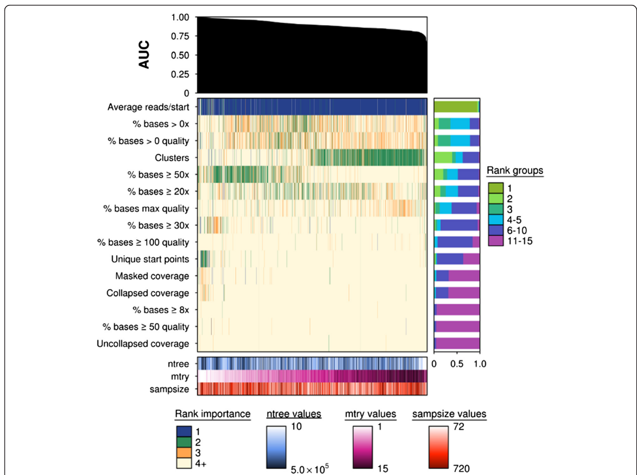
Fig. 4 Importance ranks can be sensitive to parameter changes in low p/n studies. Summary of the variable importance ranks for each sequencing metric ( n = 15 ). An AUC plot is provided at the top indicating the relative performance of each model, represented by each column. Each model was fitted from a unique combination of n_{tree} ( n = 10 ), m_{try} ( n = 15 ) and sampsize parameters ( n = 10 ) and their respective outcomes (importance value) for each metric. Each column of the main heatmap corresponds to a model's importance values, and were ranked from 1–15, where 1 represented the most important feature and 15 the least. The importance values were ordered according to previously calculated AUC scores using predicted vote and true class labels. Each row represents a metric and are ordered according to the mean rank of its importance values. The importance values were simplified in the main heatmap and illustrate four groups only. Blue indicates a rank of 1, green a rank of 2, gold a rank of 3, and beige a rank of 4 and greater. A summary of overall rank groups for a particular metric are illustrated in a barplot on the right of the main heatmap and a covariate heatmap with all parameter combinations is illustrated at the bottom of the plot. The n_{tree} parameter is illustrated in blue , m_{try} in pink and sampsize in orange . Some parameters demonstrate robust behaviour to parameter changes such as “Uncollapsed coverage” and “% bases \geq 50 quality”, which were ranked between 11–15 inclusive in 96 % and 95 % of all samples, respectively. These variables possessed VIMs that suggested they were less influential on classification accuracy. Yet, “Average reads/starts” was insensitive to parameter changes and was considered the most important variable. Another variable “Clusters” was parameter sensitive, illustrating that variables vary in their sensitivity to parameter changes which can ultimately influence classification accuracy
