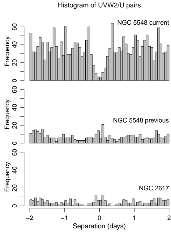
FIG. 1.— Histograms showing the number of UVW2/U pairs for the current intensive NGC 5548 monitoring campaign (top), the earlier NGC 5548 campaign (middle, McHardy et al. 2014) and the NGC 2617 campaign (bottom, Shappee et al. 2014). Data are binned by orbit, and all pairs with separations of less than half an orbit are excluded. UVW2 was used because it was the most frequently observed UVOT band, while U , a typical less well sampled band, was used because that band is particularly interesting (see Section 4.2). The range \pm 2 days is shown because this is the key cadence range that has not previously been well sampled. Note that the current campaign samples these short cadences \sim 5 -8 times more frequently than the previous NGC 5548 and NGC 2617 campaigns.
