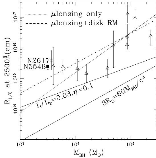
FIG. 6.— Accretion disk size estimates from quasar microlensing studies (open triangles, Mosquera et al. 2013), the current study of NGC 5548 (black filled square) and NGC 2617 (open square, Shappee et al. 2014) as a function of black hole mass. The dotted line shows the fit to just the microlensing data and the dashed line the fit to all data points including the Seyfert 1 RM measurements. To give a sense of other scales associated with accretion disks, the lower solid line shows the last stable orbit of a non-rotating black hole at R = 3R_{\text{Sch}} = 6GM/c^2 and the upper solid lines shows R_{1/2} at 2500Å for a simple thin disk with Eddington ratio L/L_{\text{Edd}} = 0.03 and efficiency \eta = 0.1 to provide a sense of scale. The latter curve can be shifted as (L/L_{\text{Edd}})^{1/3} for different choices of these factors.
