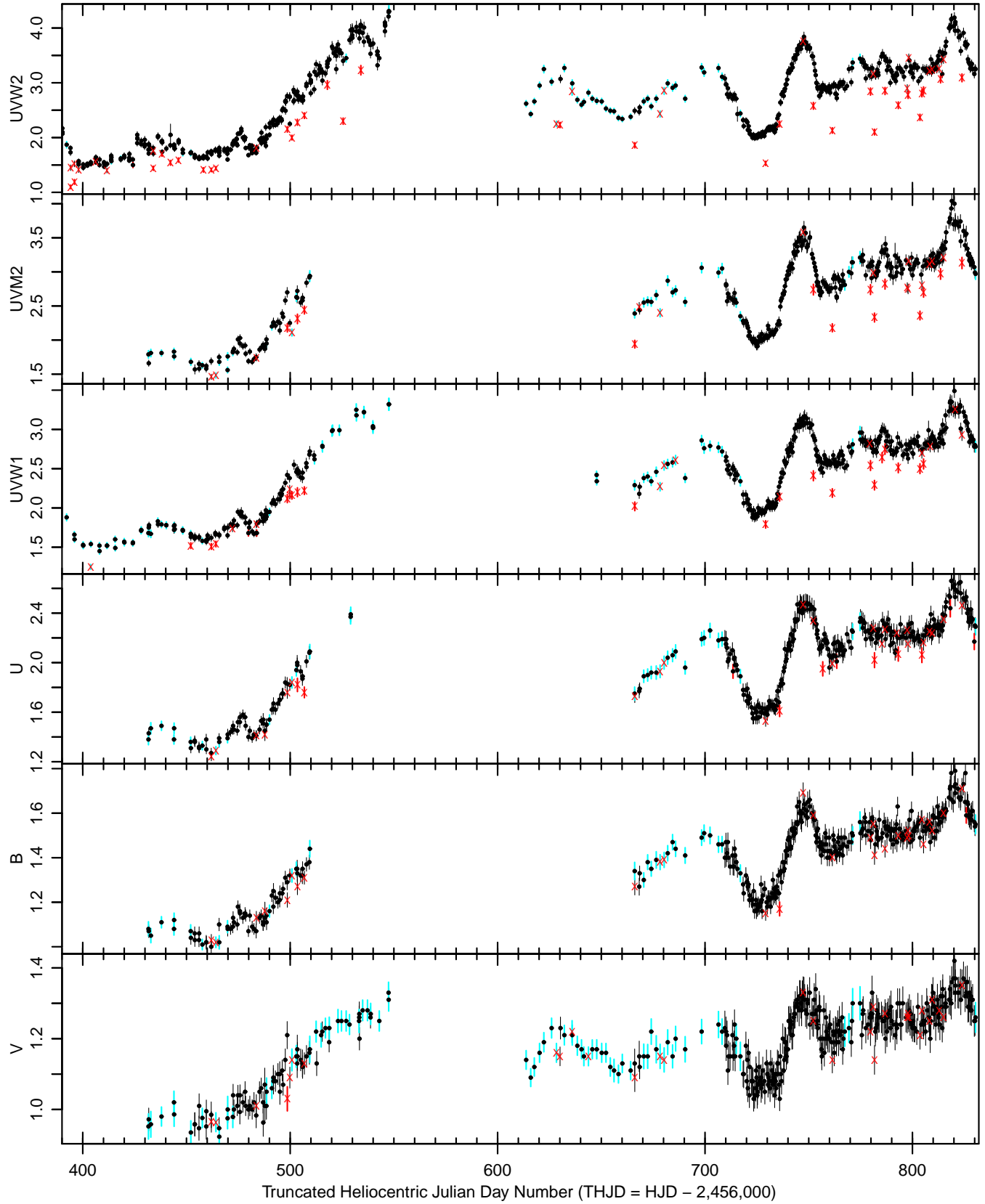
FIG. A1.— Initial UVOT light curves of NGC 5548 for the period THJD 390-832. The error bar colors indicate the results of the dropout test: black errors indicated that the point passed the dropout test (small deviation), red error bars indicated that it failed the test (large deviation) and cyan error bars indicate that it was not tested (as it lacked sufficient nearby neighbors). The symbols show if the point fell inside/outside the UVOT boxes (shown in Figure A3): black dots fell outside the boxes and thus were used in the final light curve (shown in Figure 1) and red Xs fell inside the boxes and were excluded from the final light curves.
