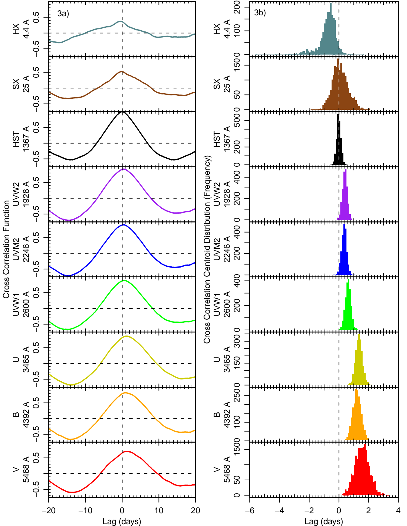
FIG. 3.— (3a) Interpolated cross-correlation functions for the intensive monitoring period light curves (Figure 2), with all correlations measured relative to the HST light curve, after removing long term trending (see Section 3). The band name and central wavelength are given on the left of each panel. Note that the interband lag goes from negative to increasingly positive as the band’s wavelength increases. Note also that the UV/optical correlations are all strong ( r_{max} = 0.57 - 0.90 ) but the X-ray/UV correlations are much weaker, ( r_{max} < 0.45 ). (3b) Cross-correlation centroid histograms derived from the CCFs as discussed in the text. The band name and central wavelength are given on the left of each panel. All distributions except HX appear consistent with a Gaussian.
