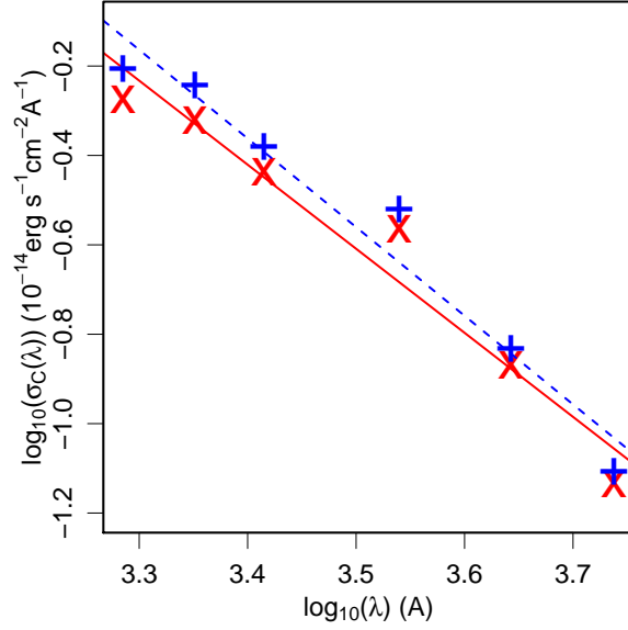
FIG. 5.— The error-subtracted variable flux ( \sigma_C(\lambda) ) as a function of wavelength ( \lambda ). The original data are shown as red Xs and the dereddened data as blue crosses. A fit to the function \log_{10}(\sigma_C(\lambda)) = \alpha \log_{10}(\lambda) + \beta yielded \alpha = -1.88 \pm 0.20 for the original data (solid red line) and \alpha = -1.98 \pm 0.20 for the dereddened data (dashed blue line).
