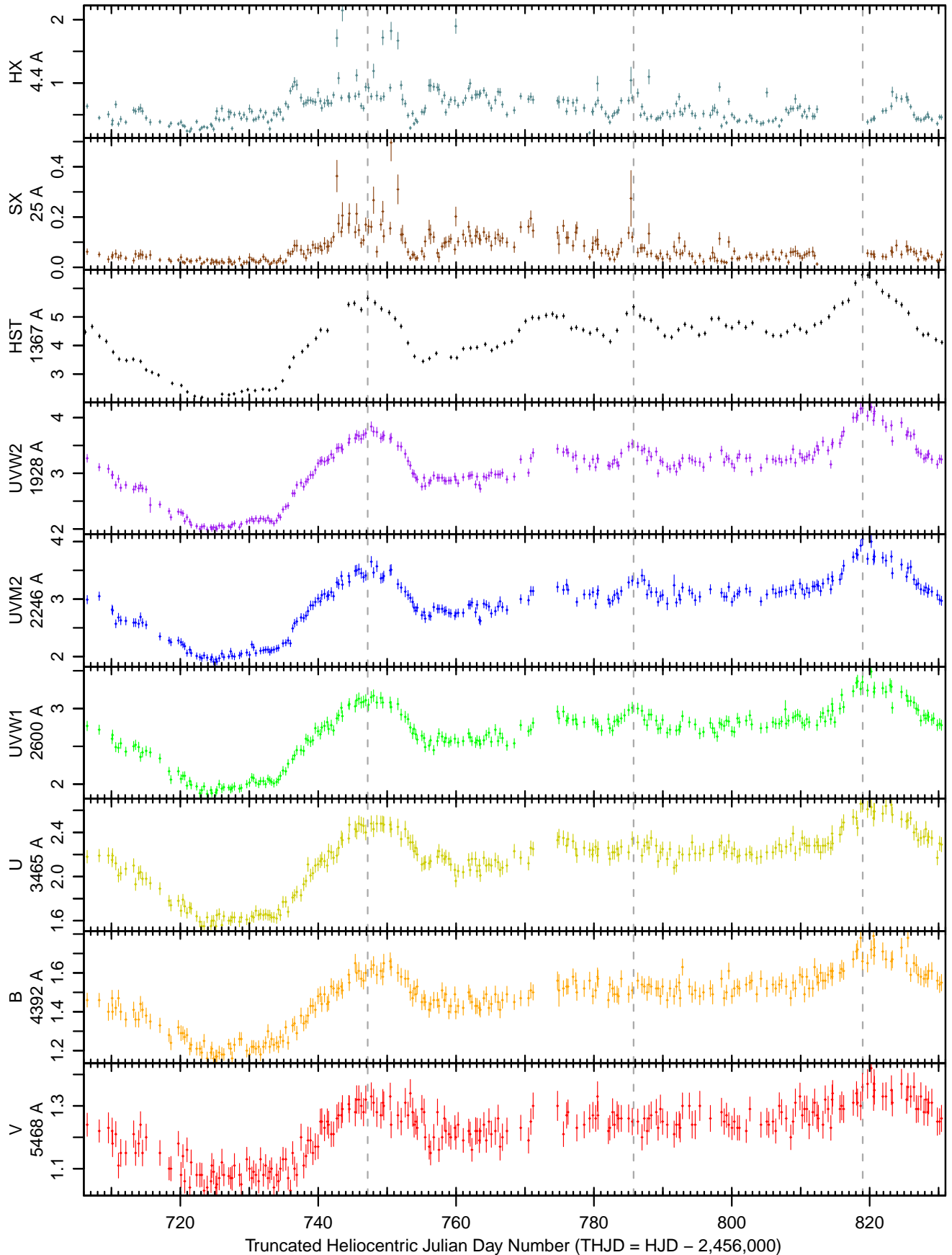
FIG. 2.— Light curves for the intensive monitoring period (HJD 2,456,706-2,456,831), going from shortest wavelength (top) to longest (bottom). The band name and central wavelength are given on the left of each panel. Top two panels show the Swift hard and soft X-ray (HX and SX respectively) light curves, in units of c/s . Third panel shows the HST light curve, in units of 10^{-14} \text{ ergs}^{-1} \text{ cm}^{-2} \text{ \AA}^{-1} . Error bars for this light curve are typically \sim 1.5\% , just barely visible in the plot. The bottom six panels show the Swift light curves, again in units of 10^{-14} \text{ erg cm}^{-2} \text{ s}^{-1} \text{ \AA}^{-1} . Dashed gray lines show times THJD 747.179, 785.752 and 818.993, three local maxima of the HST light curve.
