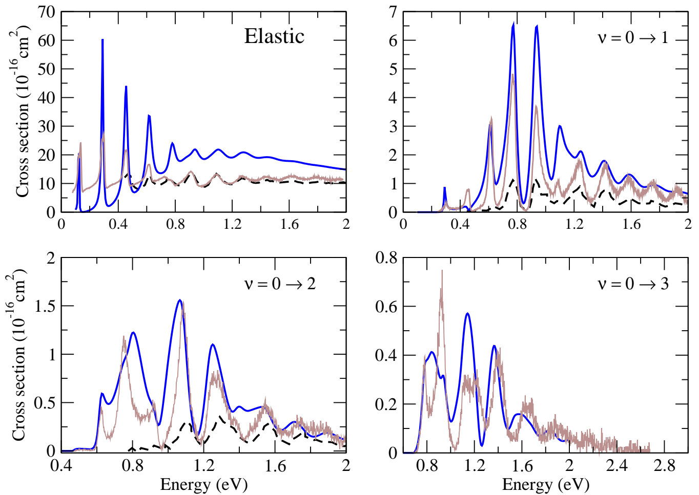
FIG. 4: Comparison of theory and experiment for elastic and vibrationally excited cross sections. Solid dark curves: present results; dashed curves: experimental measurements of Jelisavcic et al. [8]; solid grey curves: experimental measurements of Allan \times 4\pi [13].
