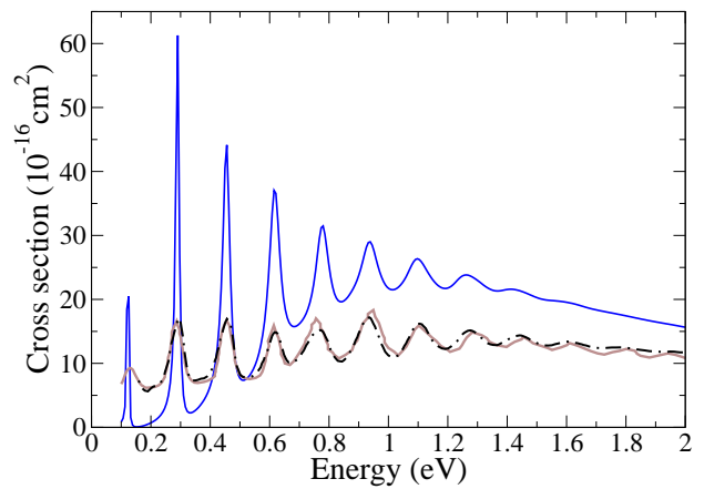
FIG. 6: Comparison of theory and experiment for grand total cross sections. Solid dark curve: present results; dash-dot curve: experimental measurements of Alle et al. [5]; solid grey curve: experimental measurements of Zecca et al. [32].
