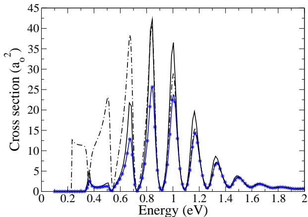
FIG. 2: {}^3\Sigma^- symmetry component of the e^- -NO \nu = 0 \rightarrow 1 vibrational excitation cross section. Comparison of different theoretical models for treating the nuclear dynamics. Solid curve: nonlocal model; solid curve with stars: local complex potential model with inclusion of barrier penetration factors; dash-dot: local complex potential (boomerang) model.
