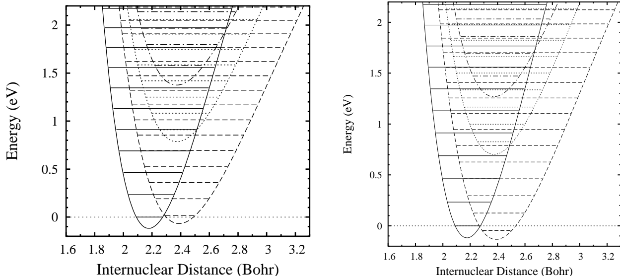
FIG. 1: NO and NO - potential curves and vibrational levels. Solid curves: 2 Π neutral ground-state; dashed curves: 3 Σ - anion; dotted curves: 1 Δ anion; dash-dot curves: 1 Σ + anion. Left panel: curves obtained from configuration-interaction calculations; right panel: shifted CI curves (see text).
