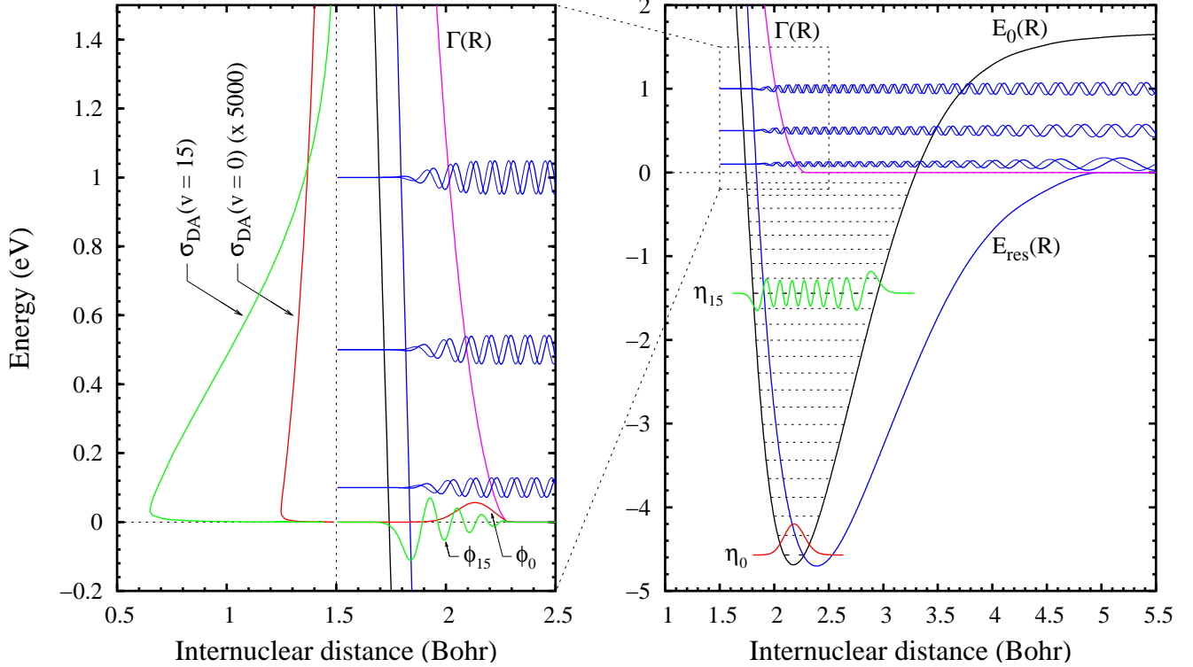
FIG. 8: Right panel: Potential energy curves of NO and of the ^3\Sigma^- resonance (solid curves), and vibrational levels of the neutral target (dotted lines). Also shown are the vibrational wave functions \eta_0(R) and \eta_{15}(R) and the scattering solution of Eq. (22), \psi_E , at E = 0.1, 0.5 and 1.0 eV (solid curves). Left panel: enlargement of the selected region of the right panel. In addition to the wave functions mentioned above, the entry amplitudes \phi_0(R) and \phi_{15}(R) (see Eq.(6)) are shown. Vibrationally excited DA cross sections are plotted for \nu = 0 ( \sigma_{DA}(\nu = 0) \times 5000 ), and for \nu = 15 ( \sigma_{DA}(\nu = 15) ).
