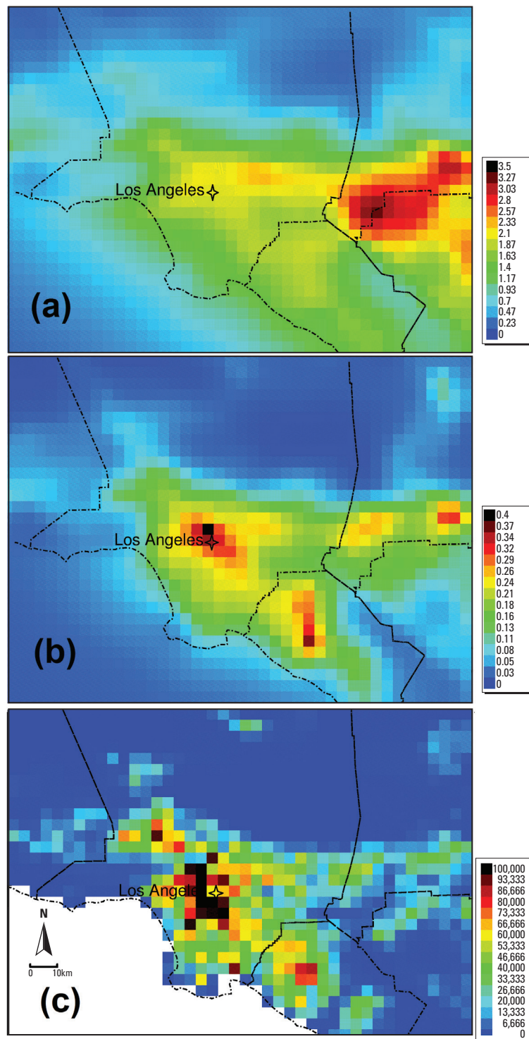
Figure 1. Modeled concentrations ( \mu\text{g}/\text{m}^3 ) of PM 2.5 nitrate (A), ultrafine anthropogenic secondary organic aerosols (B), and population in the Los Angeles Basin (C) using 4-km grids (the star in the figures indicates the site of the U.S. EPA monitor).
