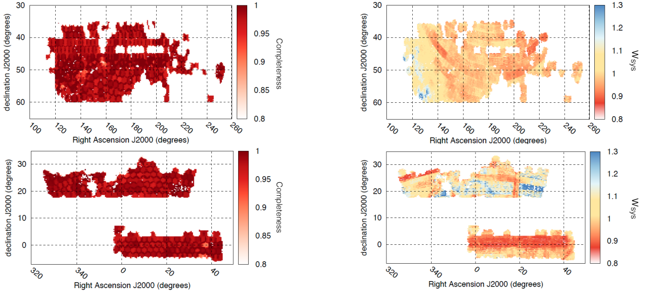
Figure 3. Angular footprint of the DR14Q sample for the NGC (top panels) and SGC (bottom panels), where the colour mapping indicates the completeness, C_{eBOSS} (see Eq. 6), and the imaging weight, w_{sys} , (see Eq. 4), in the left and right panels, respectively.
