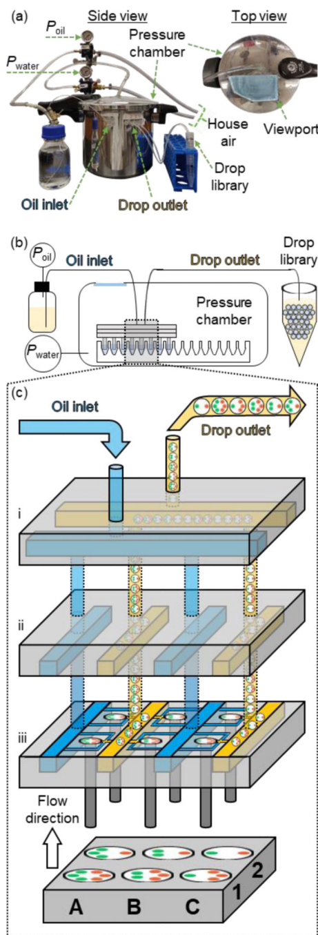
Fig. 2. PIPE chip operation and barcoded drop library production. (a) Side view and top view profiles of the PIPE chip apparatus and components. (b) PIPE chip operation schematic for the encapsulation of 96 wells from a 384-well microtiter plate. Pressure P_{oil} is applied to an external oil reservoir to provide oil to the device within the pressure chamber while a second pressure P_{water} applied to the chamber pushes fluid from sample wells into the microfluidic device. Barcoded drops travel through tubing past a sealed opening in the wall of the chamber for collection in a drop library. (c) Detailed schematic of the internal channels
