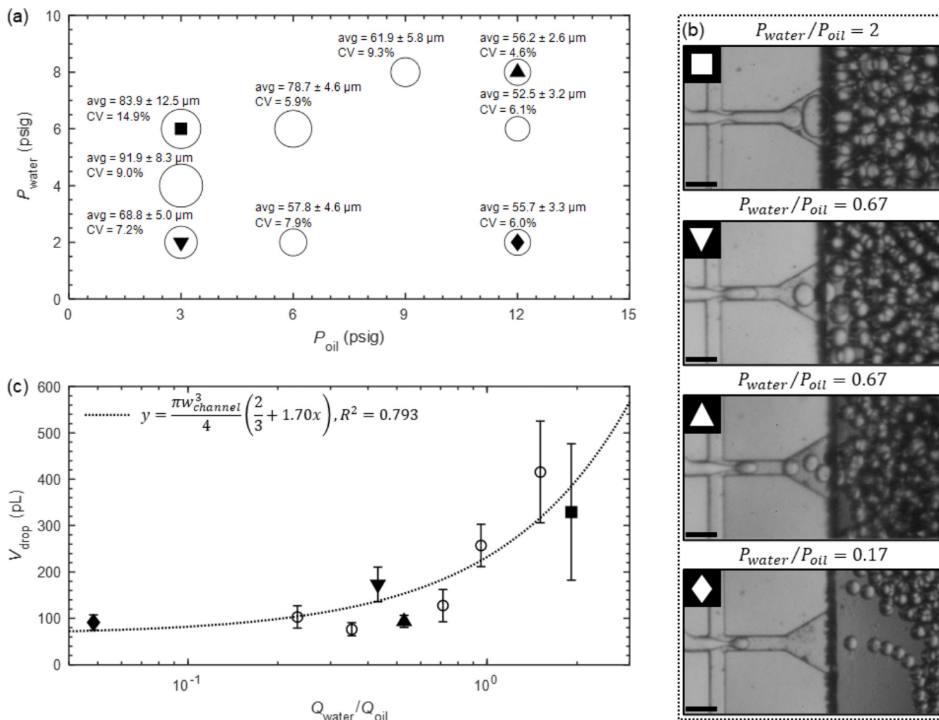
Fig. 3. Characterization of drop sizes produced by the PIPE chip. (a) Drop diameter average, standard deviation, and CV at various water pressures P_{\text{water}} and oil pressures P_{\text{oil}} . For additional visualization, the relative size of each open circle corresponds to the relative mean drop diameter measured. Solid shapes indicate conditions used for high-speed image capture in (b). (b) High-speed image capture of drop formation, ordered by descending D_{\text{drop}} , for high water pressure (■, P_{\text{water}} = 6 psig and P_{\text{oil}} = 3 psig, P_{\text{water}}/P_{\text{oil}} = 2 ), low combined pressure (▼, P_{\text{water}} = 2 psig and P_{\text{oil}} = 3 psig, P_{\text{water}}/P_{\text{oil}} = 0.67 ), high combined pressure (▲, P_{\text{water}} = 8 and P_{\text{oil}} = 12 psig, P_{\text{water}}/P_{\text{oil}} = 0.67 ), and high oil pressure (◆, P_{\text{water}} = 2 psig and P_{\text{oil}} = 12 psig, P_{\text{water}}/P_{\text{oil}} = 0.17 ) conditions. Scale bars = 100 \mu\text{m} . (c) Corresponding drop volumes V_{\text{drop}} versus the volumetric flowrate ratio Q_{\text{water}}/Q_{\text{oil}} (open circles or solid shapes). V_{\text{drop}} scales with Q_{\text{water}}/Q_{\text{oil}} following a drop scaling law (dotted black line). 34 Error bars represent one standard deviation from the mean.
