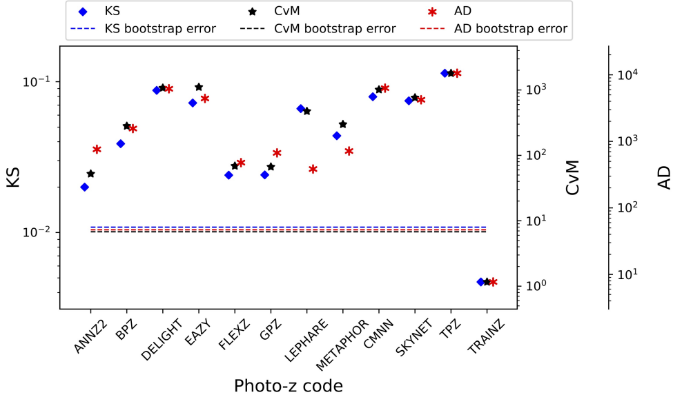
Figure 3. A visualization of the Kolmogorov-Smirnoff (KS, blue diamond), Cramer-von Mises (CvM, black star), and Anderson-Darling (AD, red asterisk) statistics for the PIT distributions. There is generally good agreement between these statistics, with differences corresponding to the codes with outstanding catastrophic outlier rates, a reflection of the differences in how each statistic weights the tails of the distribution. Horizontal lines indicate the level of uncertainty found by bootstrapping a training set sample of 30,000 galaxies using trainZ ; none of the codes reach this conservative ideal floor in expected uncertainty.
