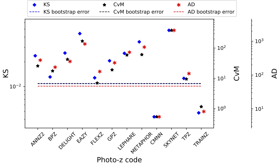
Figure A2. A visualization of the Kolmogorov-Smirnov (KS, blue diamond), Cramer-von Mises (CvM, black star), and Anderson-Darling (AD, red asterisk) statistics for the \hat{N}(z) distributions. Horizontal lines indicate the statistic values (including uncertainty) achieved using trainZ via bootstrap resampling a training set containing 30,000 redshifts. We make the reassuring observation that these related statistics do not disagree significantly with one another. CMNN outperforms the control case, trainZ , and several codes are within a factor of two of this conservative idealized limit. SkyNet scores poorly due to an overall bias in its redshift predictions.
