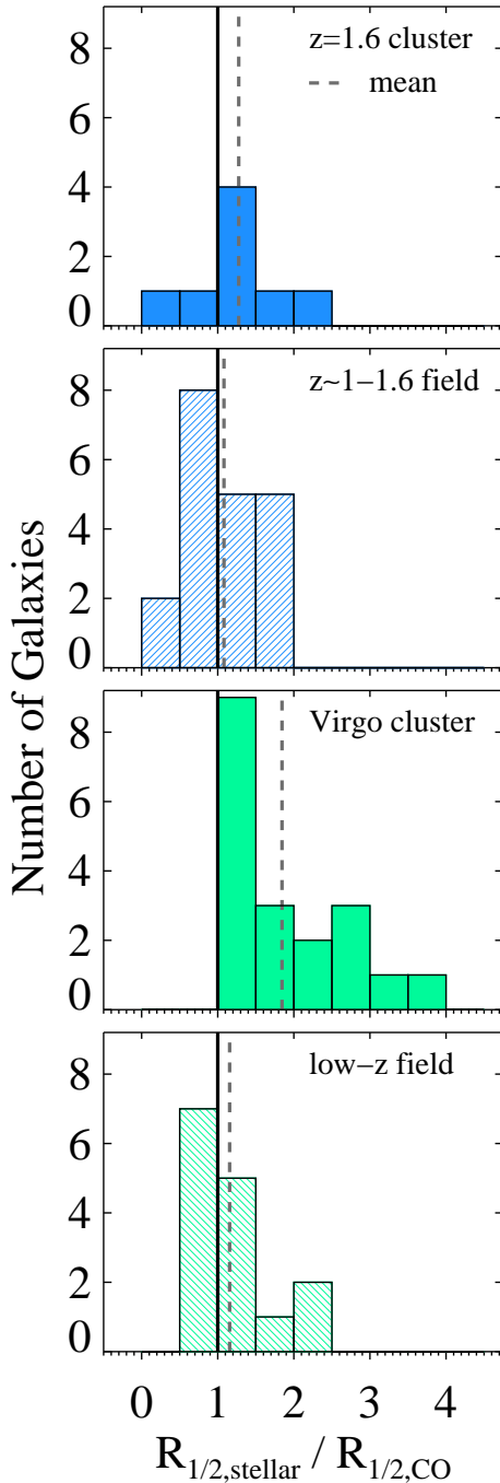
Figure 4. The ratio of the half-light radius of the optical stellar component to that of the molecular gas disk. In all panels the solid black line represents a ratio of unity, and the dashed gray line is the mean value for the given population. The top panel displays our results from J0225 for z \sim 1.6 cluster galaxies (filled blue histogram). The blue striped histogram below it is for coeval field galaxies in PHIBSS (Tacconi et al. 2013; Daddi et al. 2010). The two bottom panels represent lower- z distributions in Virgo cluster galaxies (filled green histogram, Kenney & Young 1988) and in the field (striped green histogram, Regan et al. 2001). There is a tentative trend for cluster galaxies to have smaller gas components compared to the optical stellar component both at low and high redshifts.
