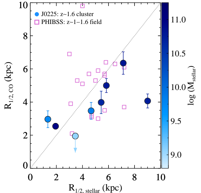
Figure 3. The half-light radii of the CO emission compared to the stellar component, measured on the rest-frame optical HST image. The z \sim 1.6 cluster galaxies in J0225 are shown as circles, color-coded by their stellar mass. The pink squares show a field comparison sample from PHIBSS (Tacconi et al. 2013; Daddi et al. 2010). Most of the galaxies fall around the dotted line, representing equal sizes for both components.
