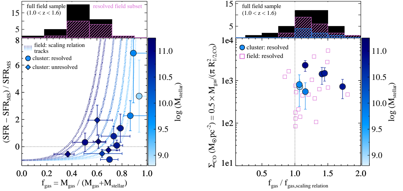
Figure 5. Left—The gas fraction as a function of offset from the star forming main-sequence for the resolved CO detections in this work (filled blue circles), and previous unresolved measurements from Noble et al. (2017) (filled diamonds). The galaxies are color-coded by their stellar mass, shown in the color bar. The field scaling relation from Genzel et al. (2015) is also shown, normalized to z = 1.6 and at a variety of stellar masses representative of the cluster sample (dashed blue lines). The upper histogram shows the gas fractions for our field comparison, with black representing the full sample, and pink representing the subset of that with resolved CO observations. Right—The molecular gas surface densities as a function of gas fraction offset from the field scaling relation, calculated for a given mass, redshift, and star formation rate. The resolved cluster (blue) and field (pink) samples are systematically above the scaling relation (represented by the gray dotted line). The upper panel shows the distribution of these subsets compared to the full field sample of resolved and unresolved detections. We note the BCG, J0225-303, lies off the x-axis range on this plot, given its high gas fraction but low star formation rate.
