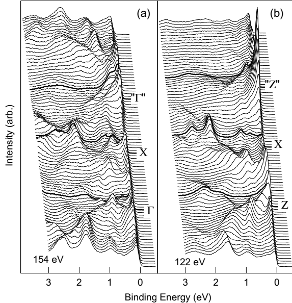
FIG. 10. Off- and on-resonance valence band spectra of \text{CeRu}_2\text{Si}_2 at (a) 154 eV and (b) 122 eV along the \langle 110 \rangle direction showing the large 4f spectral weight variations near E_F .
