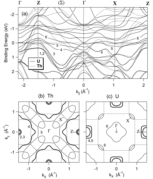
FIG. 2. Comparison of (a) theoretical LDA band structure and (b,c) 2-D Fermi-surface contours for \text{ThRu}_2\text{Si}_2 and \text{URu}_2\text{Si}_2 . Same format as Fig. 1.
