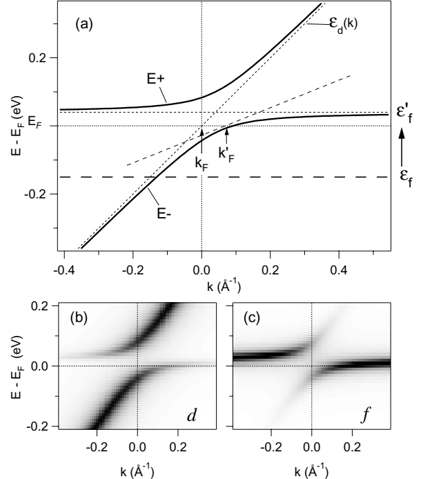
FIG. 3. (a) Schematic of the Anderson lattice model energy branches in the vicinity of a d -band crossing. (b,c) Spectral weight images illustrating the mixing of f and d -character along the two energy branches.
