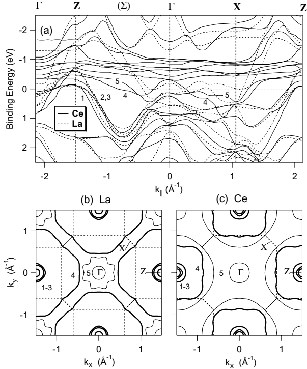
FIG. 1. Comparison of (a) theoretical LDA band structures and (b,c) 2-D Fermi-surface contours for \text{LaRu}_2\text{Si}_2 and \text{CeRu}_2\text{Si}_2 . Bold (thin) contours in (b) and (c) correspond to hole (electron) FS topologies and dashed lines are Brillouin zone boundaries. Bands that cross E_F and FS contours are numbered for clarity.
