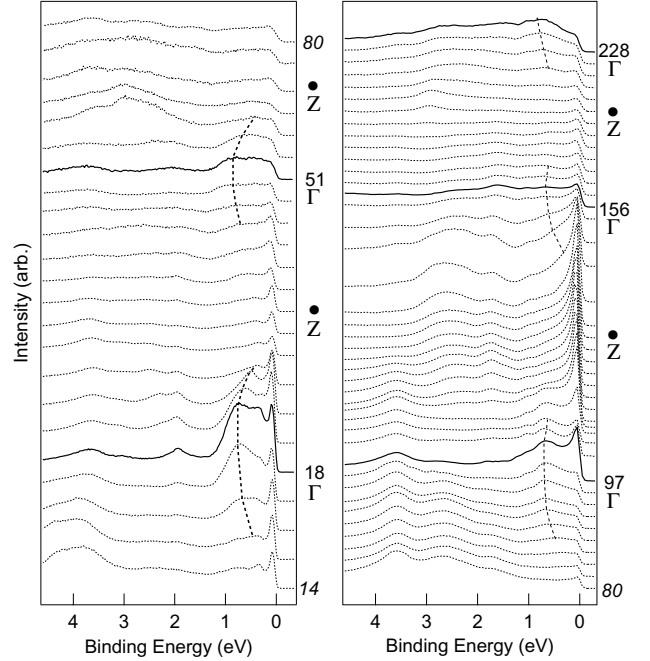
FIG. 5. Normal emission spectra of \text{URu}_2\text{Si}_2 from 14-228 eV. Dashed lines illustrate band dispersions signifying the \Gamma -points. Bullets indicate approximate spectra at Z -points.
