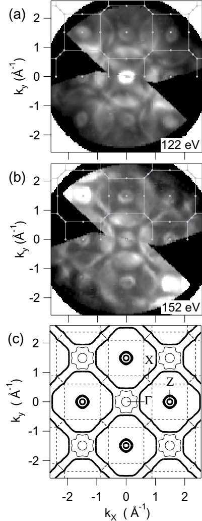
FIG. 6. Fermi-energy intensity maps of LaRu 2 Si 2 at (a) 122 eV and (b) 152 eV. Lighter grayscale is higher E_F -intensity. (c) Theoretical contours of hole (bold) and electron (fine) Fermi surface topologies.
