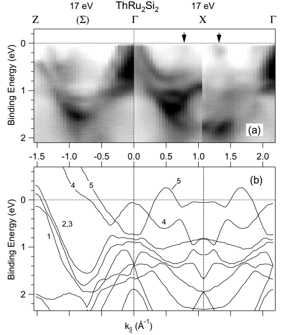
FIG. 12. (a) Valence band intensity maps of \text{ThRu}_2\text{Si}_2 at 17 eV along high-symmetry azimuth angles corresponding to \Gamma - (\Sigma) -“Z” and \Gamma -X-“ \Gamma ”. Arrows indicate the location of small electron pockets. (b) Theoretical band structure calculation for \text{ThRu}_2\text{Si}_2 .
