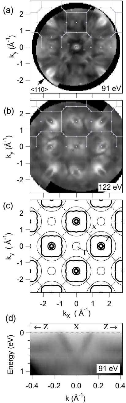
FIG. 9. Off- and on-resonance Fermi-energy intensity maps of \text{CeRu}_2\text{Si}_2 at (a) 91 eV and (b) 122 eV. (c) Theoretical contours of hole (bold) and electron (fine) Fermi surface topologies. (d) Valence band dispersion at the X-point at 91 eV orthogonal to \Gamma -X (reverse grayscale).
