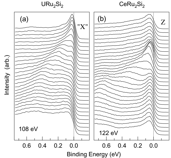
FIG. 17. High resolution on-resonance spectra near a d -band E_F -crossing for (a) URu 2 Si 2 near the X-point and (b) CeRu 2 Si 2 near the Z-point. Spectra are acquired with 0.25^\circ steps ( \Delta k \approx 0.024 \text{ \AA}^{-1} ).
