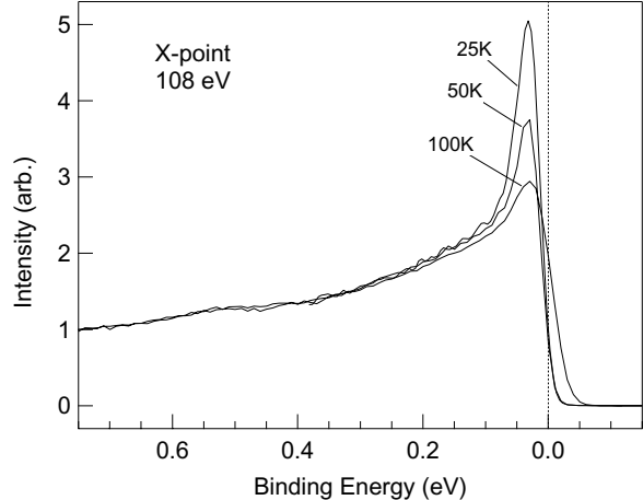
FIG. 18. Temperature dependence of angle-resolved valence spectra at 108 eV for \text{URu}_2\text{Si}_2 at the center of the “X”-point hole-pocket.
