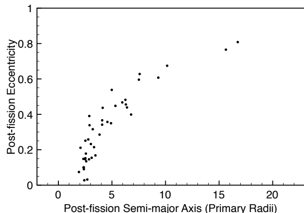
Figure 2. Results from post-fission simulations by Jacobson & Scheeres (2011) are shown after 1000 years of evolution (Seth Jacobson, personal communication, 2011).
