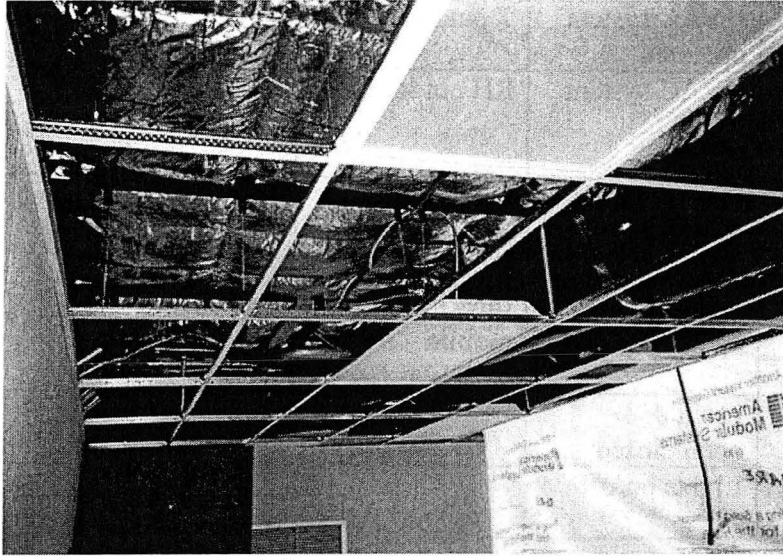
Figure 1: Photograph of the foil vapor barrier provided with roof insulation for the four HPCBS Element 6 RCs.
