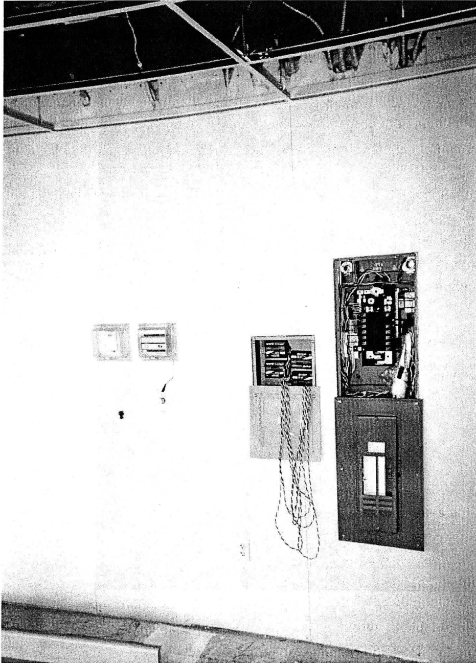
Figure 10: Photograph of P-Series WattNode digital pulse sensors (50A CT and 15A CT type), concealed in an electrical panel, used in each of the four RCs to measure total building (watt0), conventional HVAC heat pump (watt1), IDEC (watt2), and lighting (watt3) power for the electricity monitoring component of the field study.
