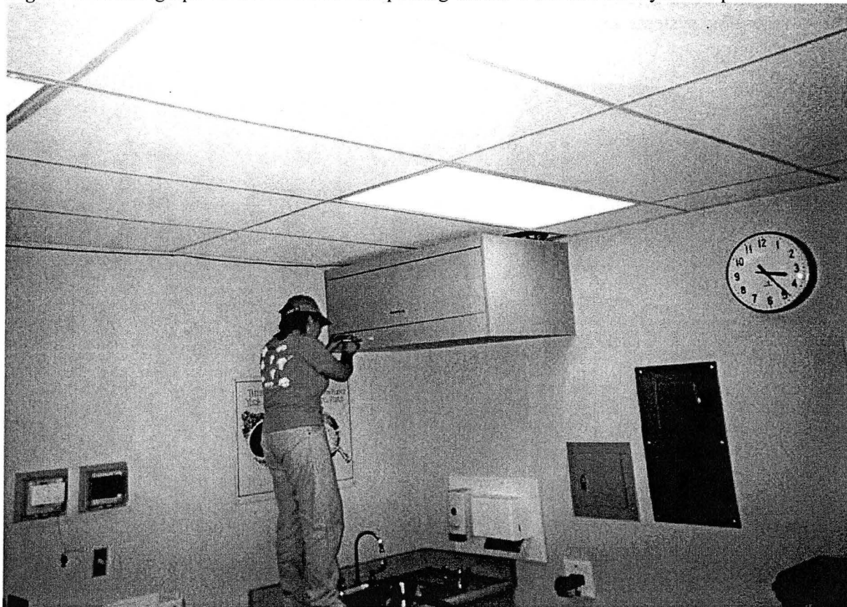
Figure 15: Photograph of LBNL technician placing indoor VOC and aldehyde samples.
