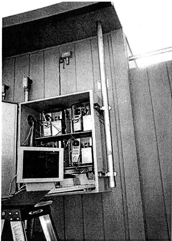
Figure 14 (a-b): Photograph of LBNL outdoor enclosure with (a) VOC and aldehyde sampling systems and (b) sampling lines for outdoor samples.
