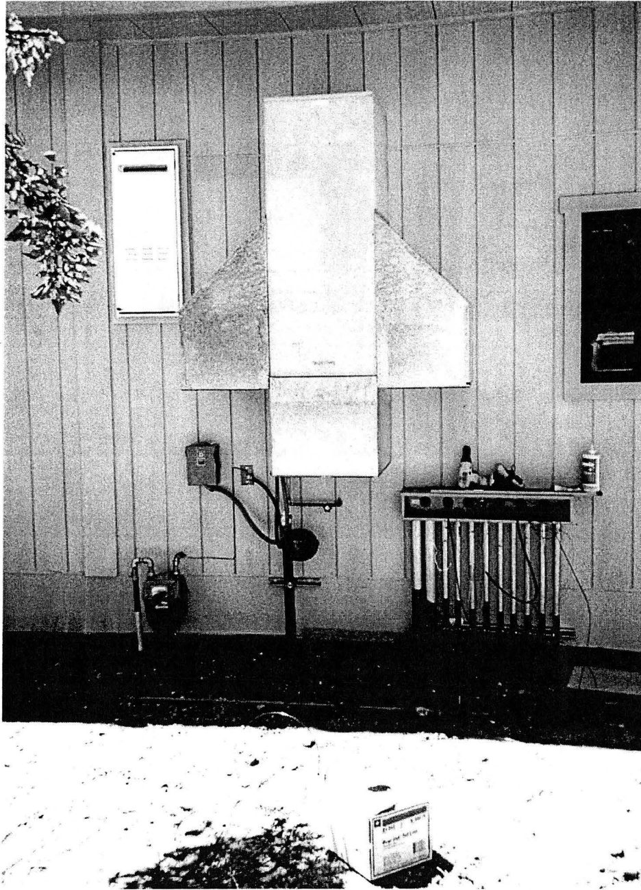
Figure 4: Photograph of the IDEC with LBNL customized inlet filtration system (65% ASHRAE dust spot efficiency DuraMax filters, two DM-603 and one DM-602, Koch Filter Corporation, Louisville, KY) mounted on the back wall of each RC.
