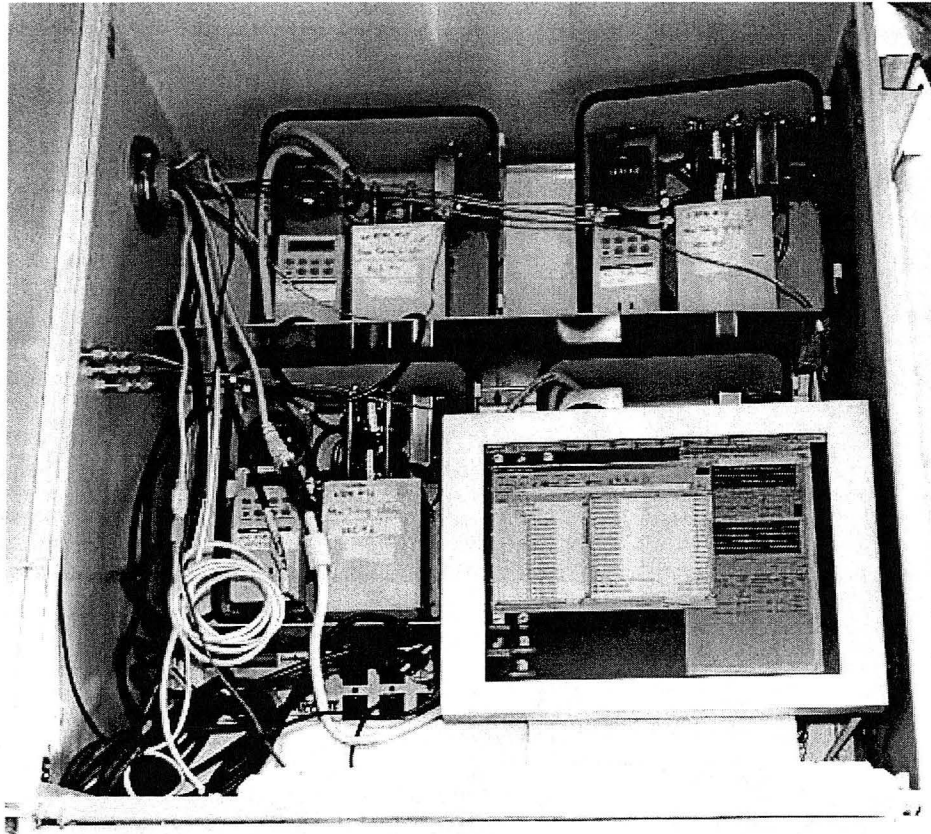
Figure 8b: Photographs of the completed (b) LBNL modified white, waterproof steel outdoor enclosure (Hoffman, Inc., San Francisco, CA) for environment monitoring and computer equipment.
