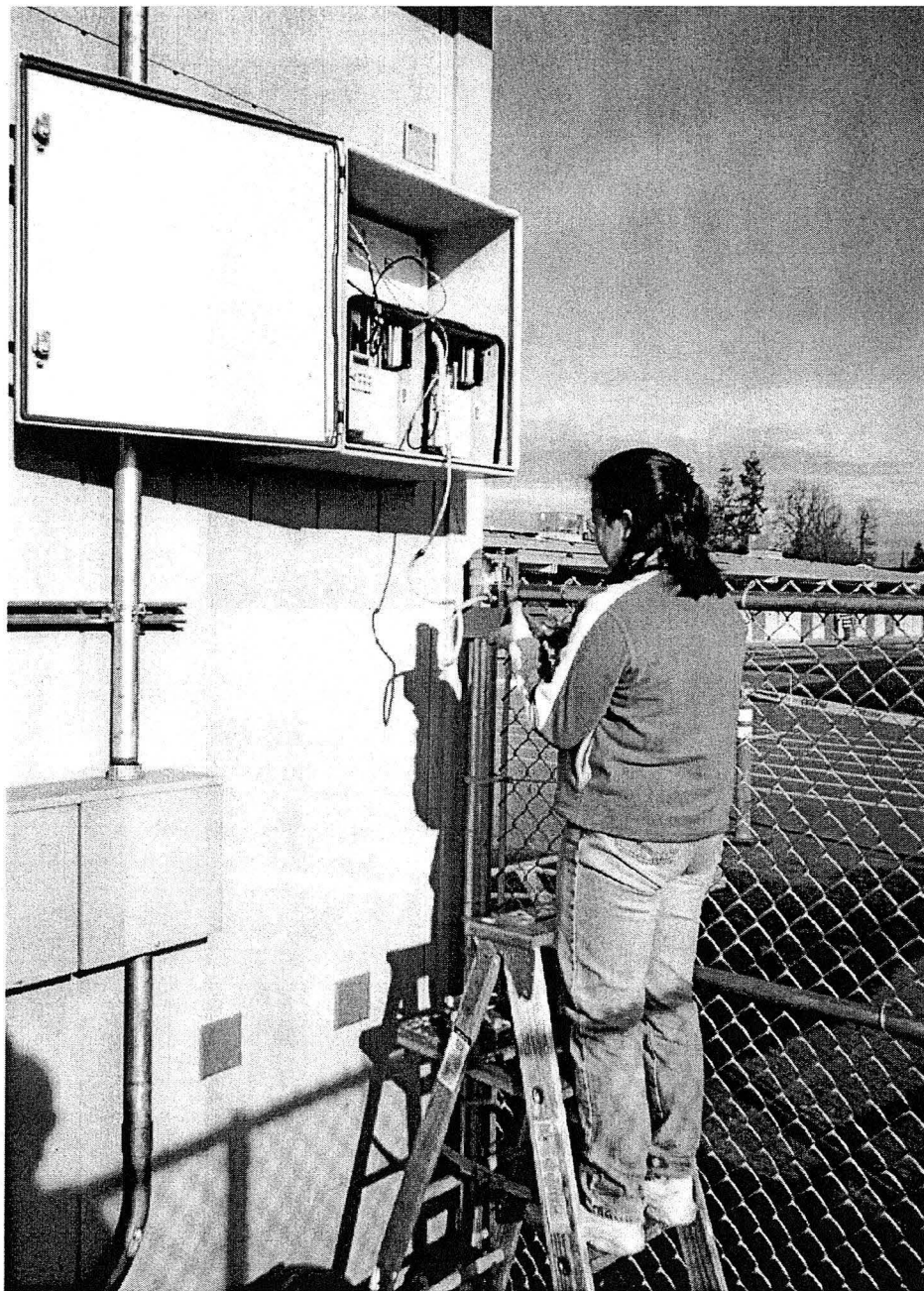
Figure 16: Photograph of LBNL technician conducting flow rate measurements of the aldehyde sampling system with a BIOS DryCal low flow cell calibrator. VOC sampling system flow rates were taken nearby with a simple bubble tube protocol.
