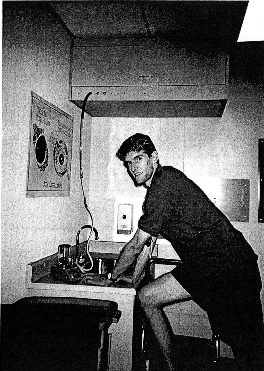
Figure 13: Photograph of LBNL technician conducting flow rate measurements of the PSI MetOne 237B particle counters with a BIOS DryCal low flow cell calibrator.
