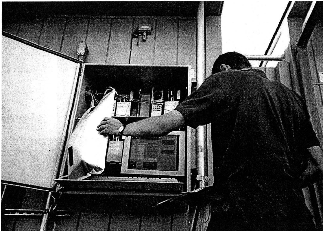
Figure 12: Photograph of LBNL technician conducting calibration protocol for CAI ZFP-9 CO 2 gas analyzers with calibration bags at percentages of 2788 ppm.
