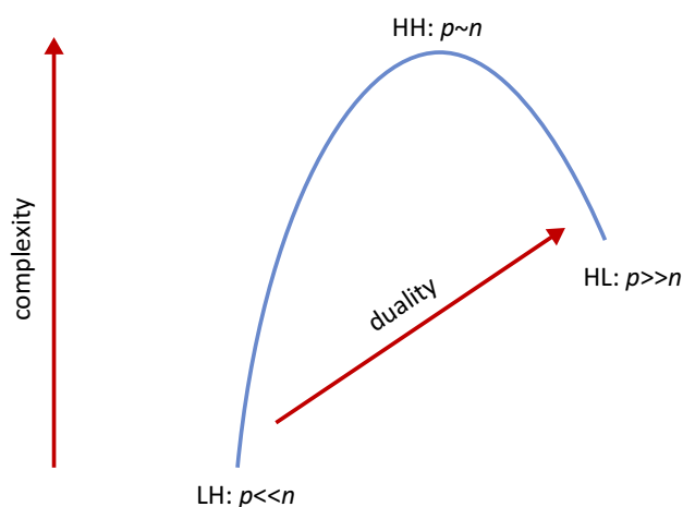
Fig. 2. Three asymptotic regimes for data analysis. LH is the low-dimension high sample size regime of classical statistics. HH is the high-dimension high sample size regime of classical random matrix theory. HL is the high-dimension low sample size regime of alternative random matrix theory. HH tends to be more complex than HL because duality arguments allow some features of classical statistics to emerge in the HL regime.
