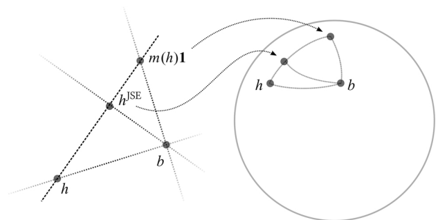
Fig. 1. Shrinkage of the sample eigenvector h along the line connecting h and m(h)\mathbf{1} in Euclidean space (Left) and projected on the unit sphere (right).
