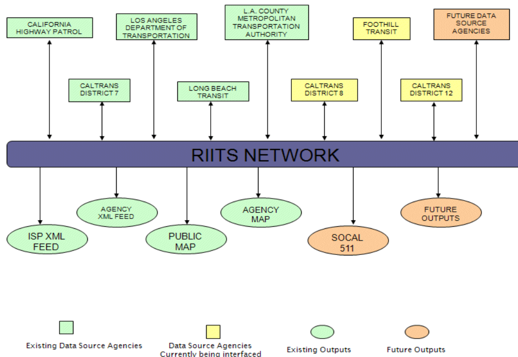
Figure 3-2 The RIITS Network: Data Providing Agencies and Outputs
