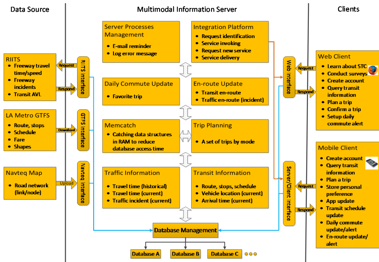
Figure 2-1 Trip2go Architecture
