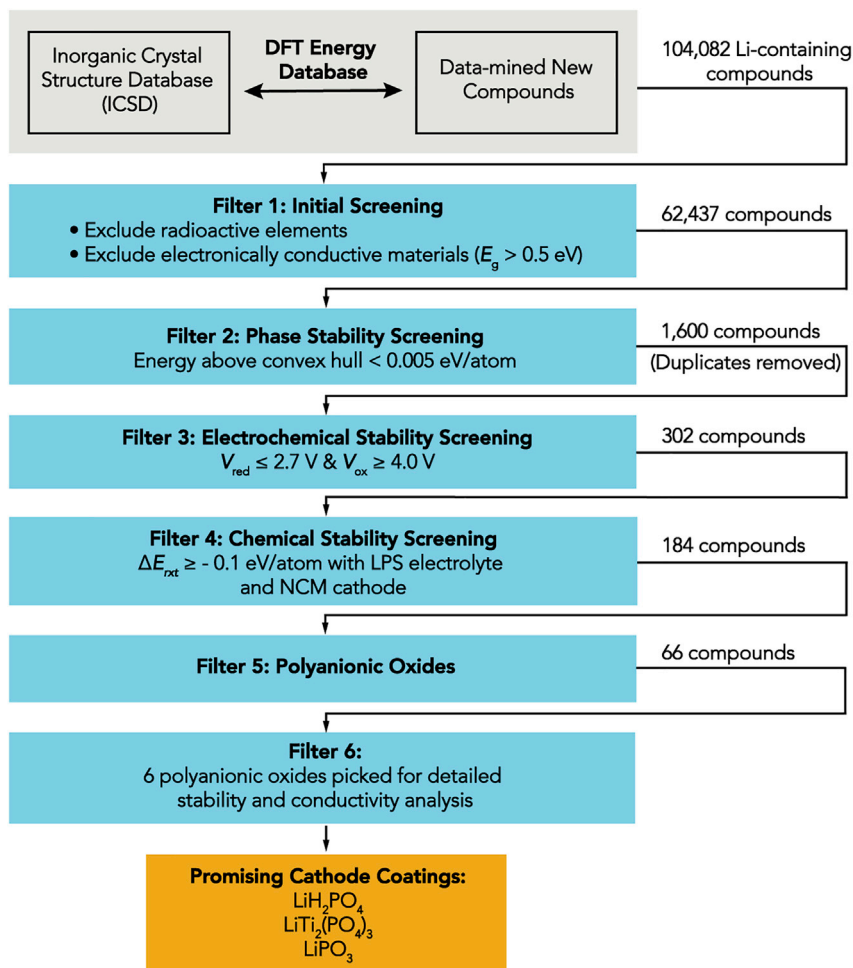
Figure 1. Flowchart Describing the Computational Screening of Cathode-Coating Materials
