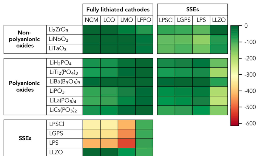
Figure 5. Reaction Energies \Delta E_{\text{rx}} at Fully Lithiated Cathode/SSE, Fully Lithiated Cathode/Coating, and Coating/SSE Interfaces in meV/atom
