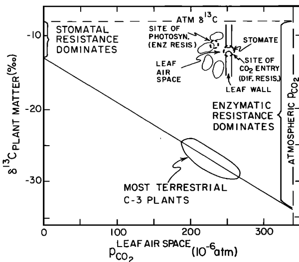
Fig. 2. Relationship between the δ 13 C for the cellulose in C-3 plants as a function of the leaf space CO 2 partial pressure (as documented by Farquhar et al. [1982]). If this pressure is near the atmospheric value, then the enzymatic fractionation dominates. If this pressure is very low, the fractionation associated with diffusion through the stomatal openings into the leaf air space must dominate. Although the exact position of the line has yet to be pinned down, the approximate trend has been established.
